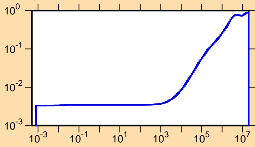
\mu vs. E for ^{203}\text{Au}(\text{mt251})
