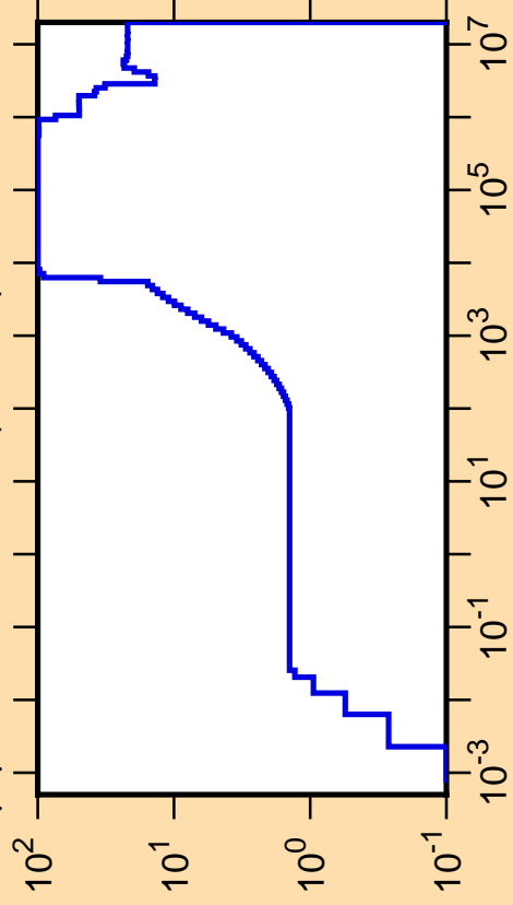
\Delta\mu/\mu vs. E for ^{203}\text{Au}(\text{mt251})
