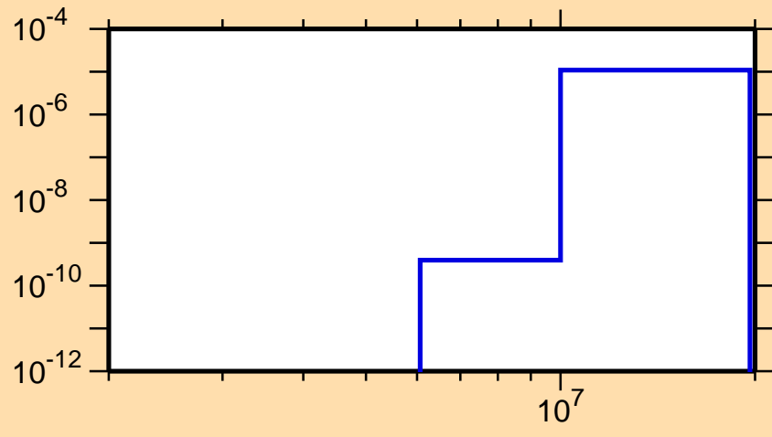
\sigma vs. E for ^{203}\text{Au}(n,\alpha)
