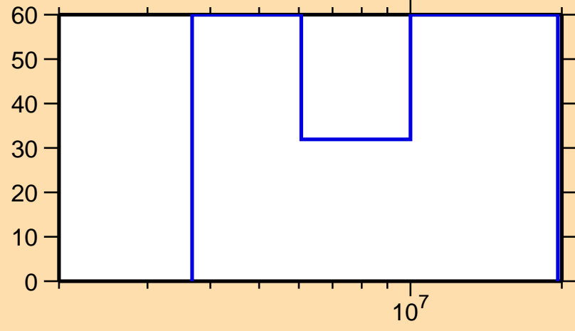
\Delta\sigma/\sigma vs. E for ^{203}\text{Au}(n,\gamma)
