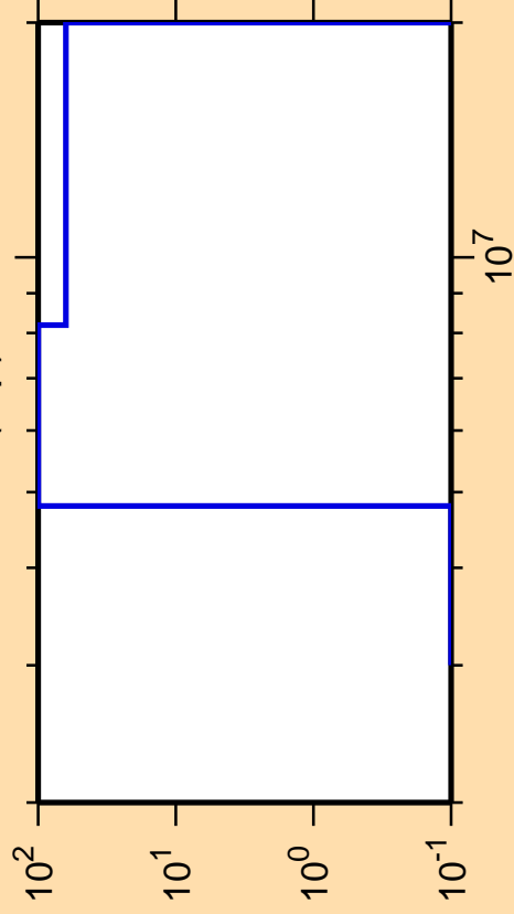
\Delta\sigma/\sigma vs. E for ^{203}\text{Au}(n,p)
