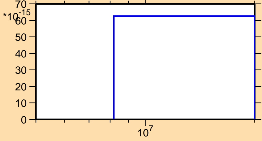
\sigma vs. E for ^{203}\text{Au}(n,2n\alpha)
