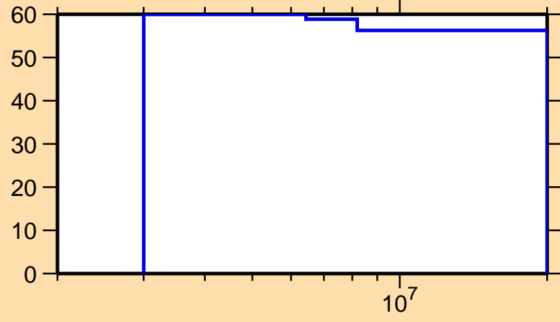
\Delta\sigma/\sigma vs. E for ^{203}\text{Au}(n,n_1)
