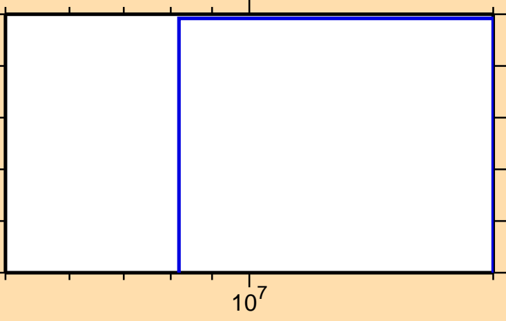
\sigma vs. E for ^{203}\text{Au}(n,n\alpha)
