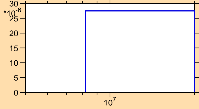
\sigma vs. E for ^{203}\text{Au}(n,d)
