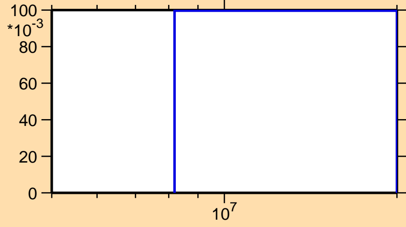
\sigma vs. E for ^{203}\text{Au}(n,3n)
