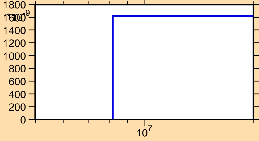
\sigma vs. E for ^{203}\text{Au}(n,t)
