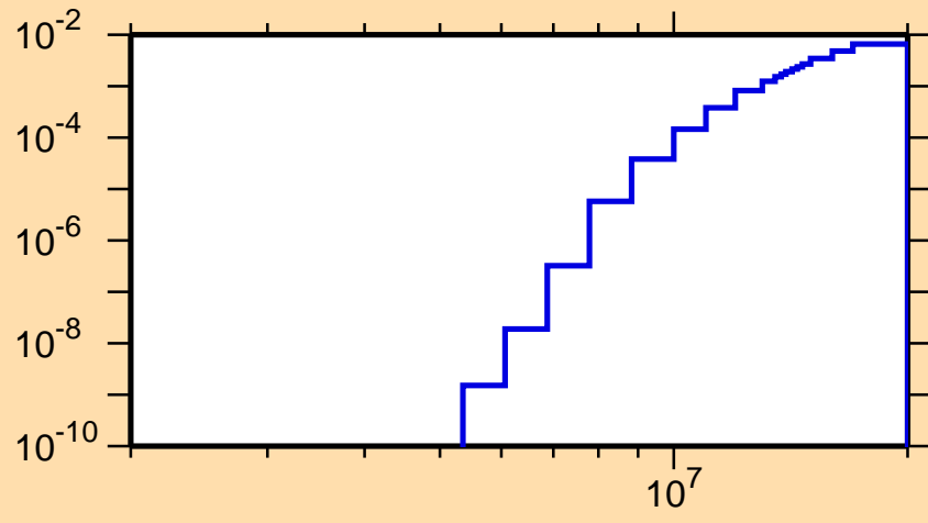
\sigma vs. E for ^{204}\text{Au}(n,p)
