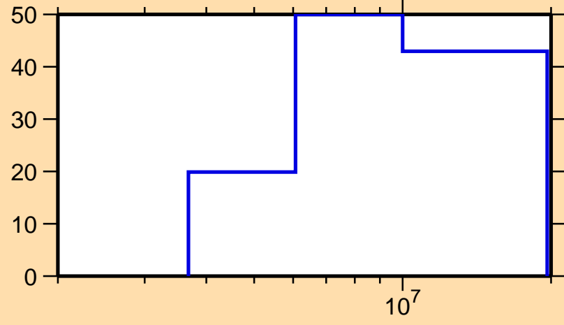
\Delta\sigma/\sigma vs. E for ^{204}\text{Au}(n,ncont.)
