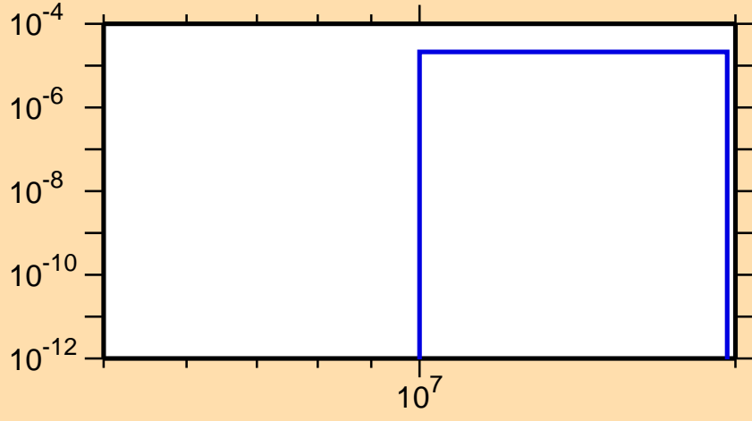
\sigma vs. E for ^{204}\text{Au}(n,d)
