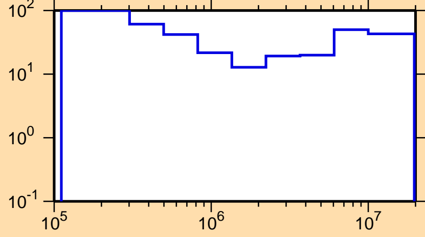
\Delta\sigma/\sigma vs. E for ^{204}\text{Au}(n,n\text{cont.})
