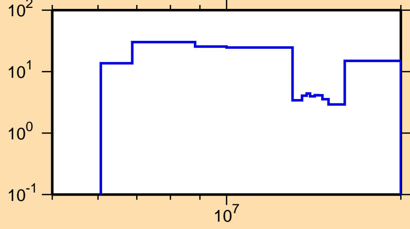
\Delta\sigma/\sigma vs. E for ^{205}\text{Au}(n,\text{el.})
