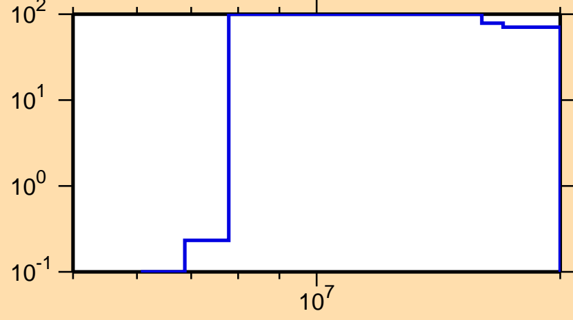
\Delta\sigma/\sigma vs. E for ^{205}\text{Au}(n,p)
