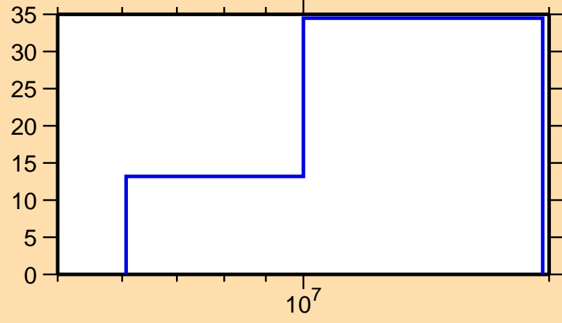
\Delta\sigma/\sigma vs. E for ^{205}\text{Au}(n,n\text{cont.})
