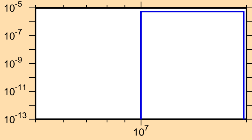
\sigma vs. E for ^{205}\text{Au}(n,np)
