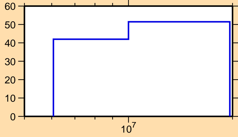
\Delta\sigma/\sigma vs. E for ^{205}\text{Au}(n,n_1)
