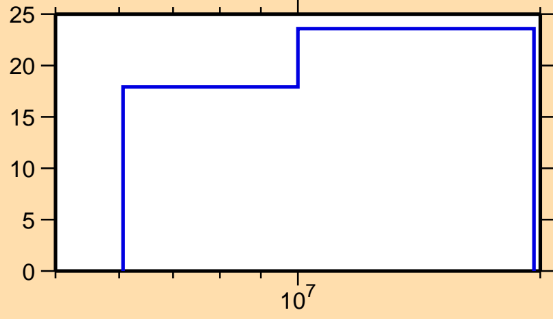
\Delta\sigma/\sigma vs. E for ^{205}\text{Au}(n,2n)
