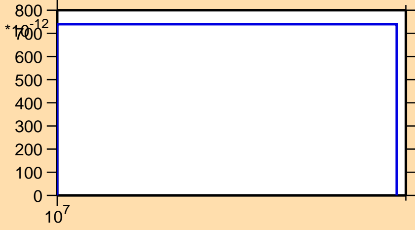
\sigma vs. E for ^{205}\text{Au}(n,nt)
