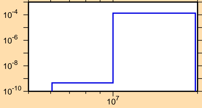
\sigma vs. E for ^{205}\text{Au}(n,p)
