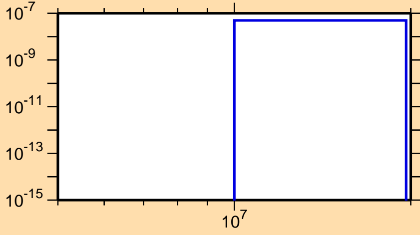
\sigma vs. E for ^{205}\text{Au}(n,n\alpha)
