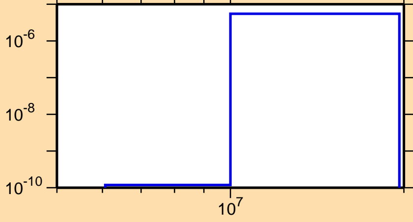
\sigma vs. E for ^{205}\text{Au}(n,\alpha)
