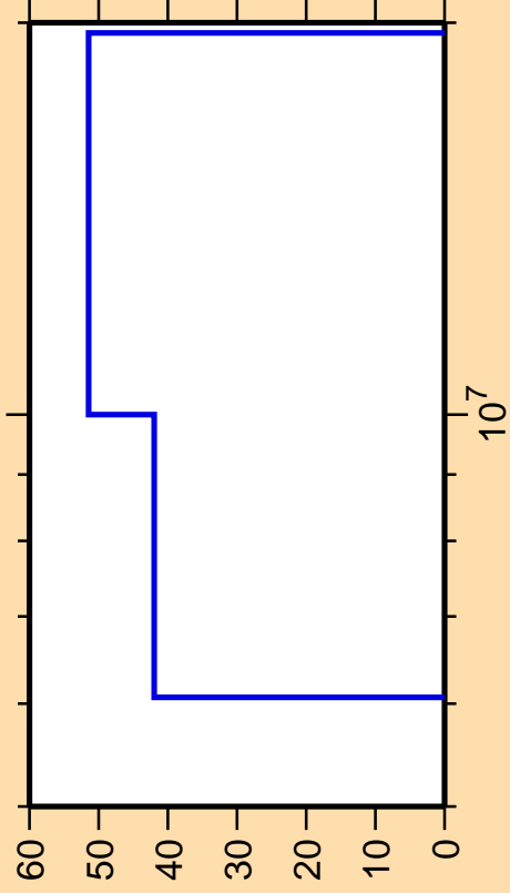
\Delta\sigma/\sigma vs. E for ^{205}\text{Au}(n,n_1)
