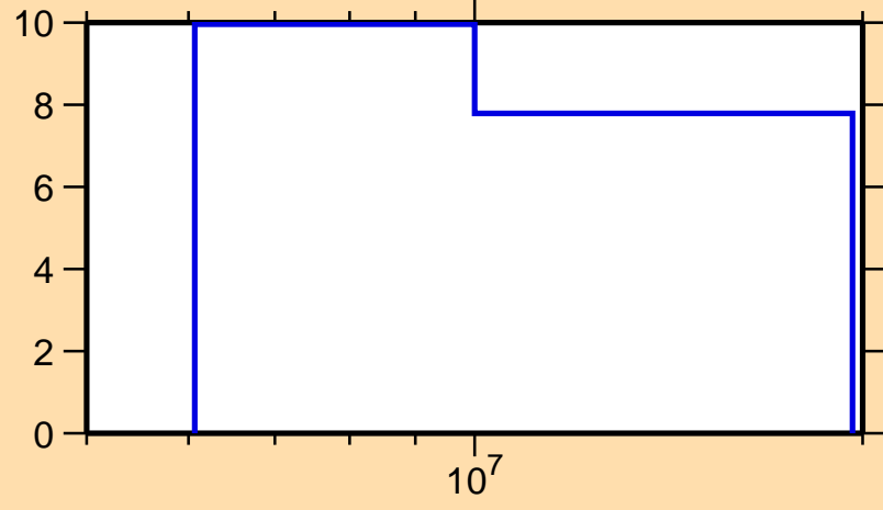
\Delta\sigma/\sigma vs. E for ^{205}\text{Au}(n,\text{nonel.})
