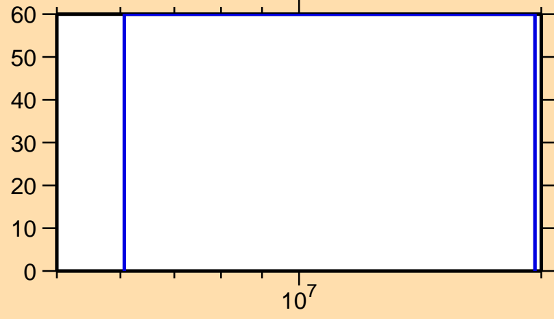
\Delta\sigma/\sigma vs. E for ^{205}\text{Au}(n,\gamma)
