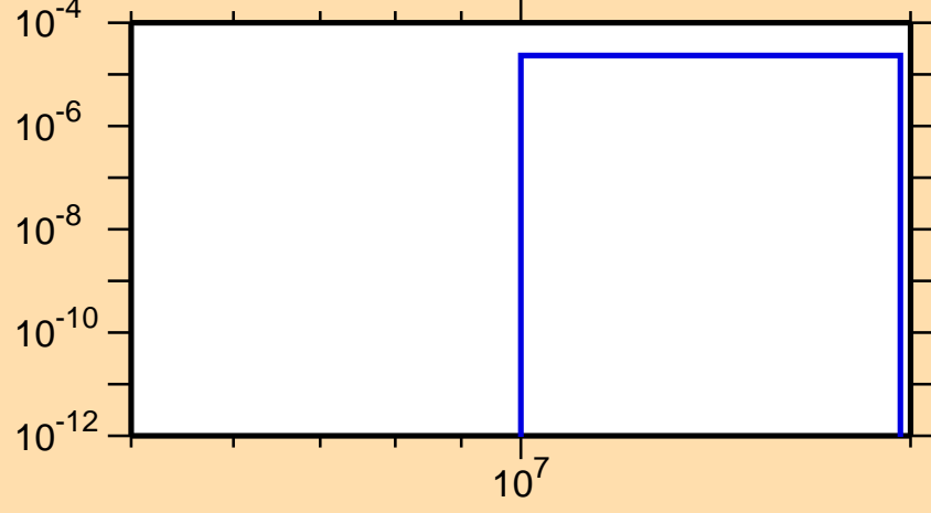
\sigma vs. E for ^{205}\text{Au}(n,d)
