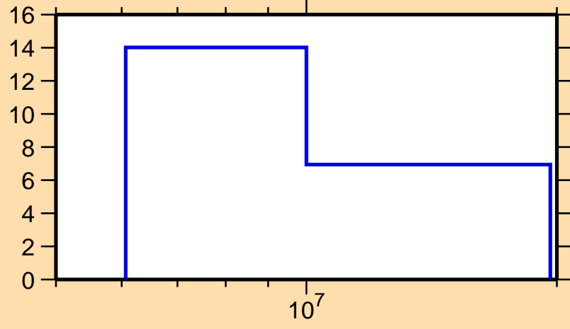
\Delta\sigma/\sigma vs. E for ^{205}\text{Au}(n,\text{tot.})
