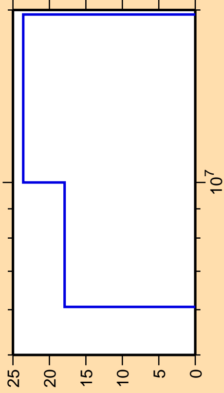
\Delta\sigma/\sigma vs. E for ^{205}\text{Au}(n,2n)
