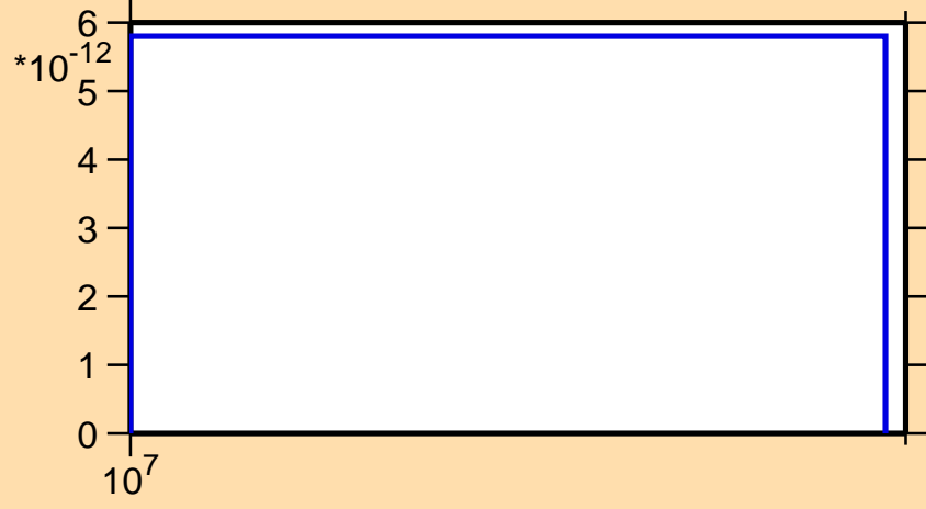
\sigma vs. E for ^{205}\text{Au}(n,2np)
