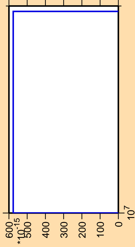
\Delta\sigma/\sigma vs. E for ^{205}\text{Au} (mt 42)
