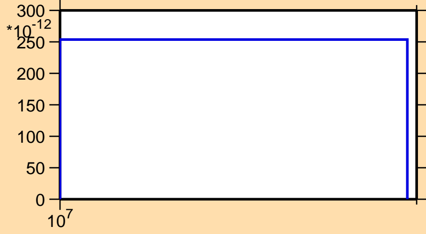
\sigma vs. E for ^{205}\text{Au}(n,\text{nd})
