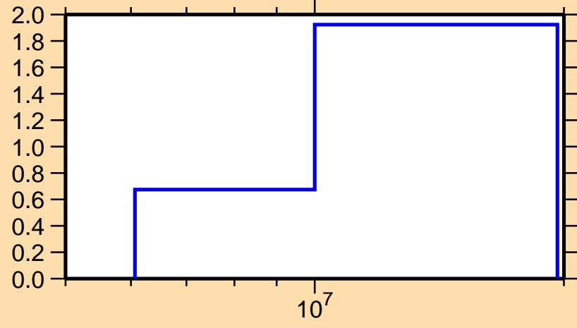
\sigma vs. E for ^{205}\text{Au}(n,2n)
