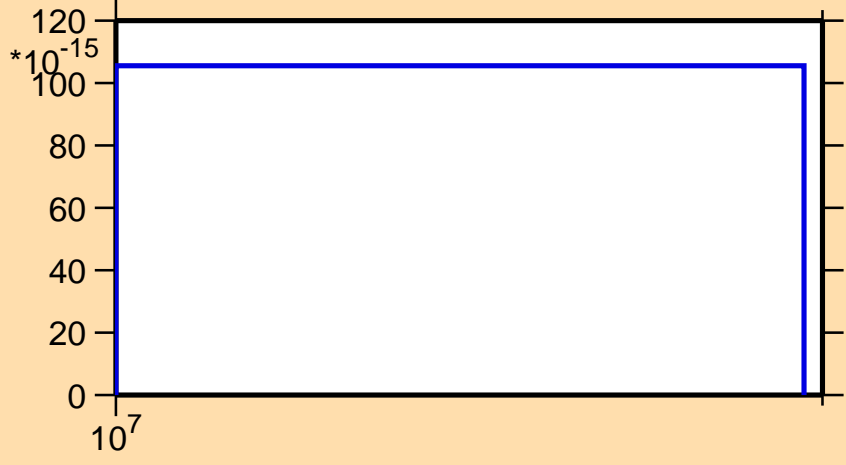
\sigma vs. E for ^{205}\text{Au}(n,2n\alpha)
