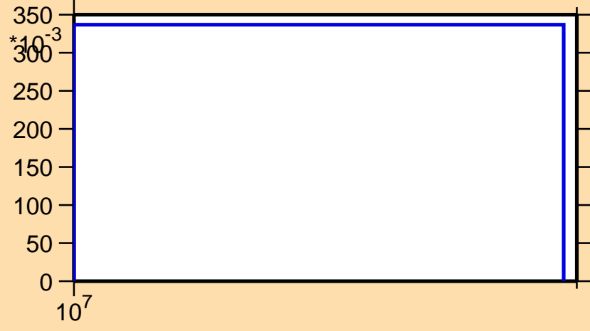
\sigma vs. E for ^{205}\text{Au}(n,3n)
