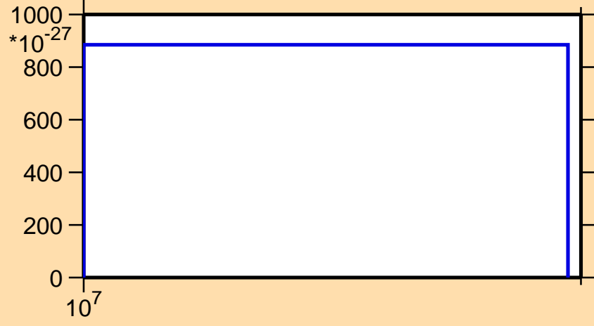
\sigma vs. E for ^{205}\text{Au} (mt 42)
