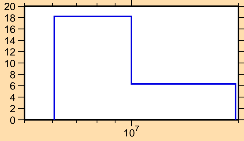
\Delta\sigma/\sigma vs. E for ^{205}\text{Au}(n,\text{el.})
