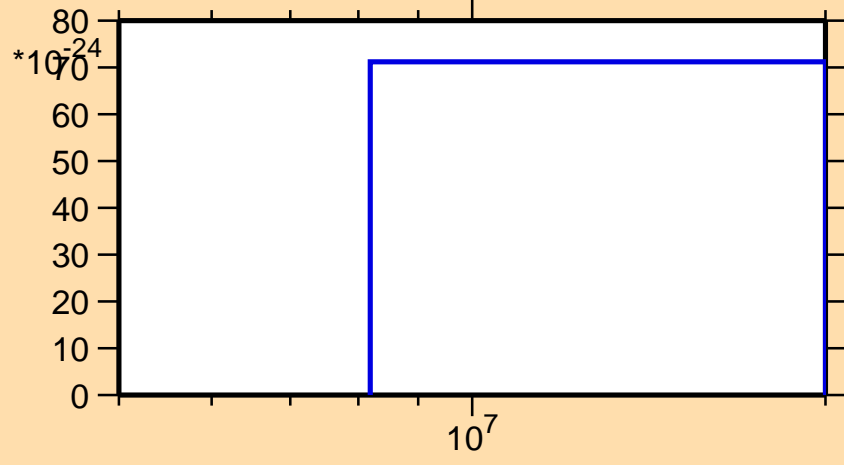
\sigma vs. E for ^{205}\text{Au}(\text{mt } 42)
