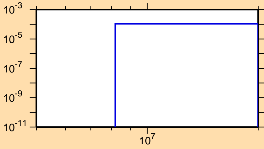
\sigma vs. E for ^{205}\text{Au}(n,p)
