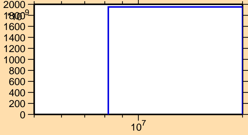
\sigma vs. E for ^{205}\text{Au}(n,t)
