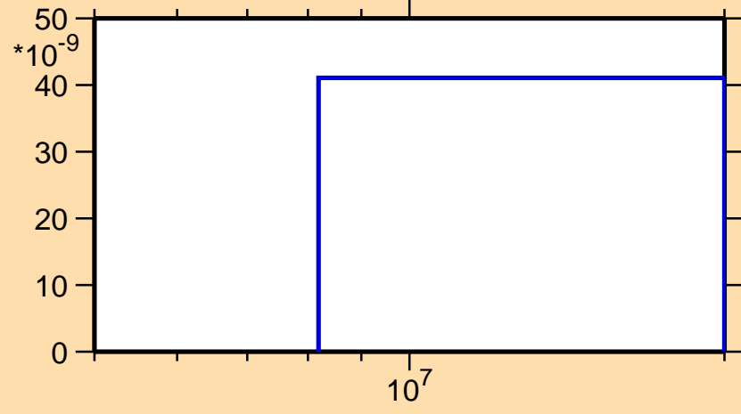
\sigma vs. E for ^{205}\text{Au}(n,n\alpha)
