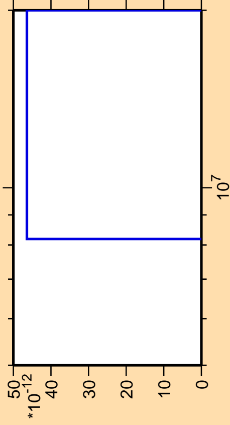
\Delta\sigma/\sigma vs. E for ^{205}\text{Au}(\text{mt } 42)
