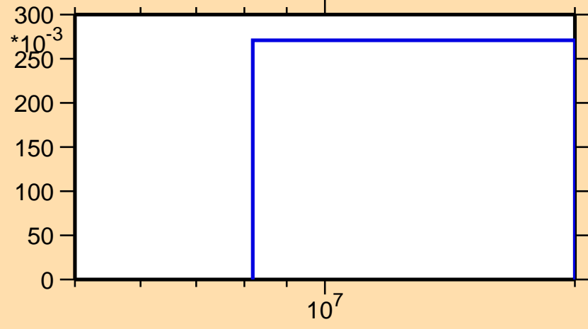
\sigma vs. E for ^{205}\text{Au}(n,3n)
