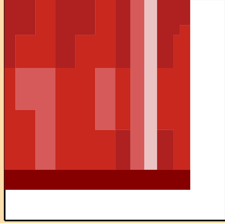
\Delta\sigma/\sigma vs. E for ^{206}\text{Au}(n,n_1)
