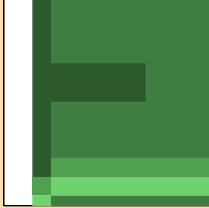
\Delta\sigma/\sigma vs. E for ^{206}\text{Au}(n,p)
