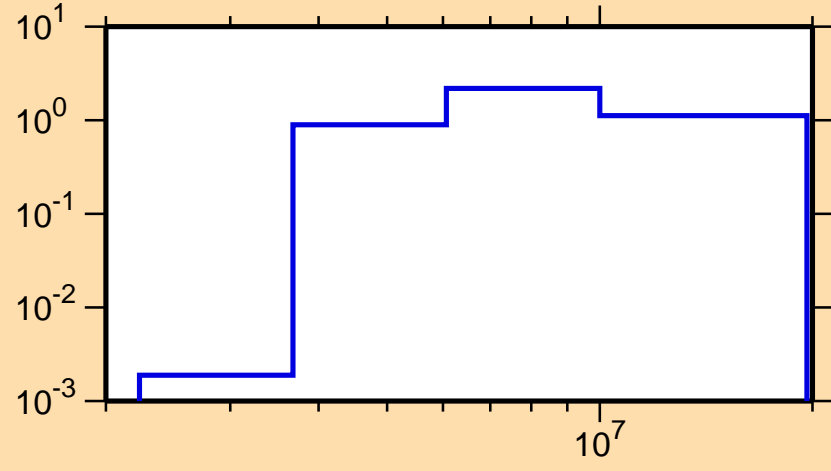
\sigma vs. E for ^{206}\text{Au}(n,2n)
