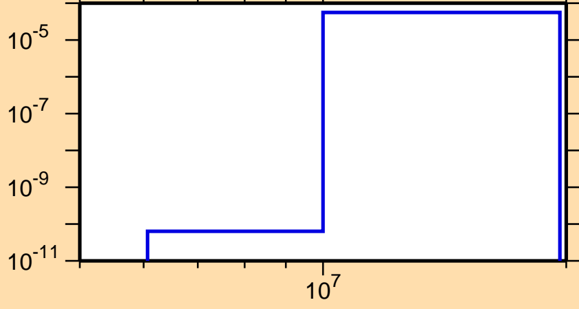
\sigma vs. E for ^{206}\text{Au}(n,t)
