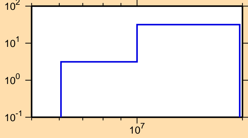
\Delta\sigma/\sigma vs. E for ^{206}\text{Au}(n,2n)
