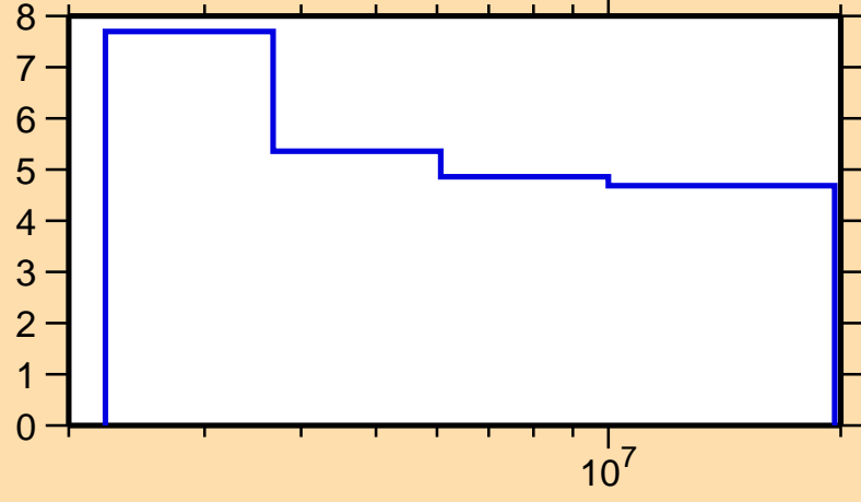
\Delta\sigma/\sigma vs. E for ^{206}\text{Au}(n,\text{nonel.})
