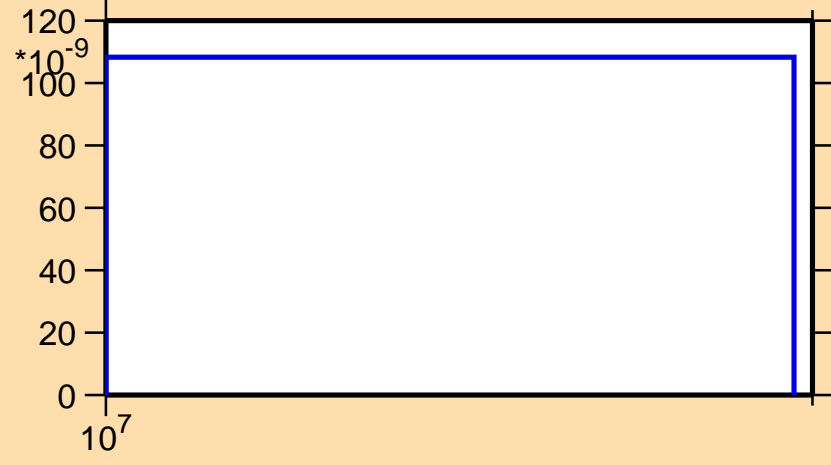
\sigma vs. E for ^{206}\text{Au}(n,nt)
