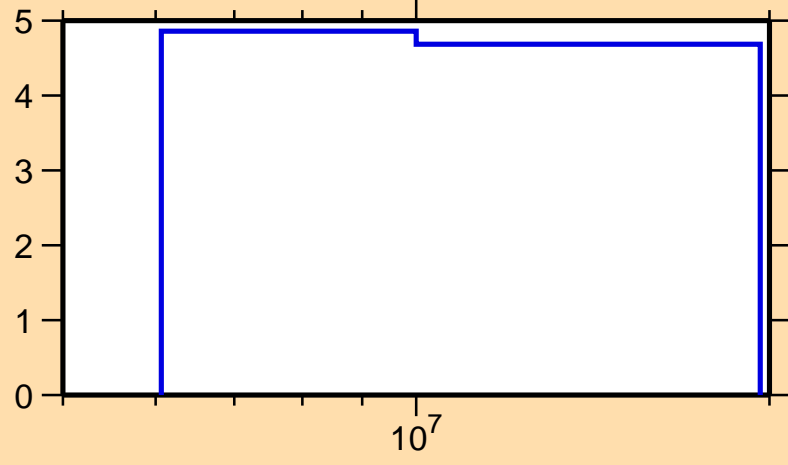
\Delta\sigma/\sigma vs. E for ^{206}\text{Au}(n,\text{nonel.})
