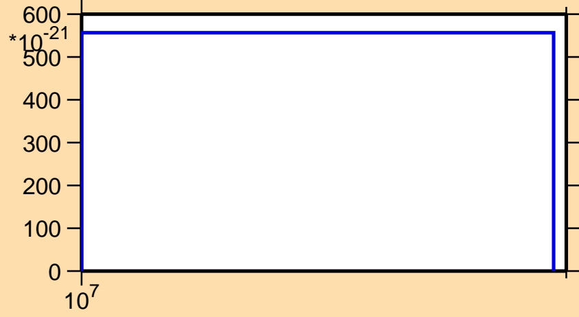
\sigma vs. E for ^{206}\text{Au}(\text{mt } 42)
