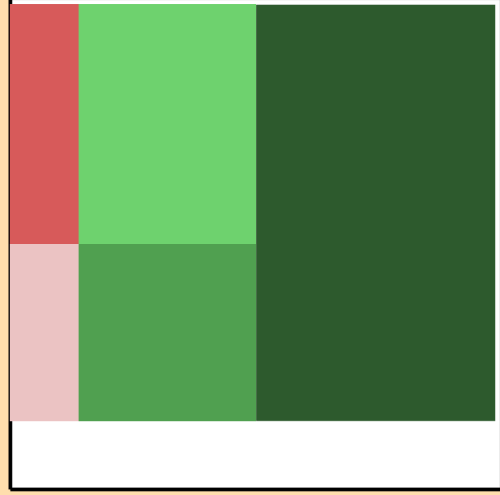
\Delta\sigma/\sigma vs. E for ^{206}\text{Au}(n,\gamma)
