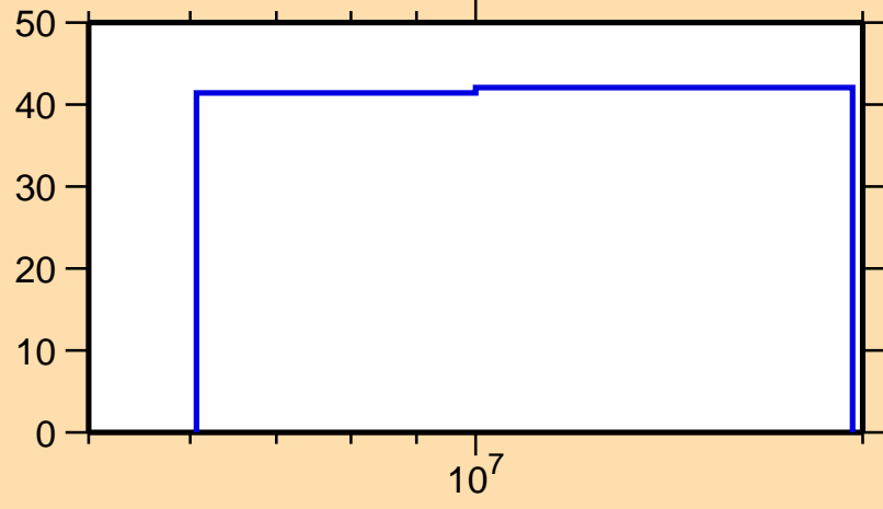
\Delta\sigma/\sigma vs. E for ^{206}\text{Au}(n,ncont.)
