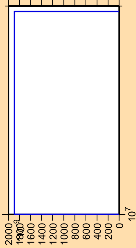
\Delta\sigma/\sigma vs. E for ^{206}\text{Au}(\text{mt } 42)
