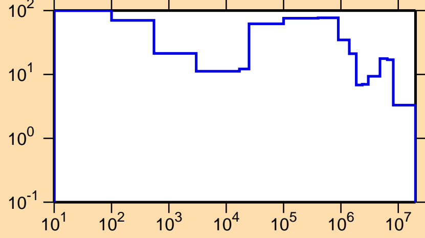
\Delta\sigma/\sigma vs. E for ^{206}\text{Au}(n,\text{tot.})
