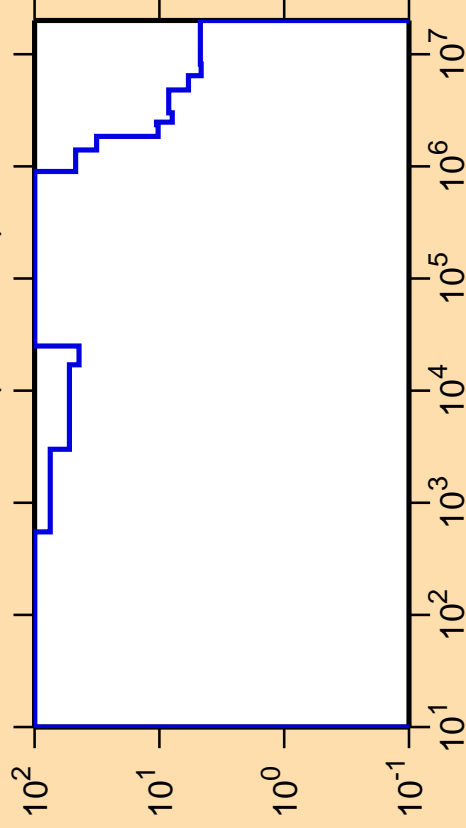
\Delta\sigma/\sigma vs. E for ^{206}\text{Au}(n,\text{nonel.})
