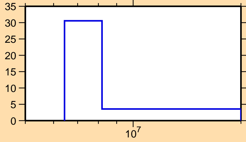
\Delta\sigma/\sigma vs. E for ^{206}\text{Au}(n,el.)
