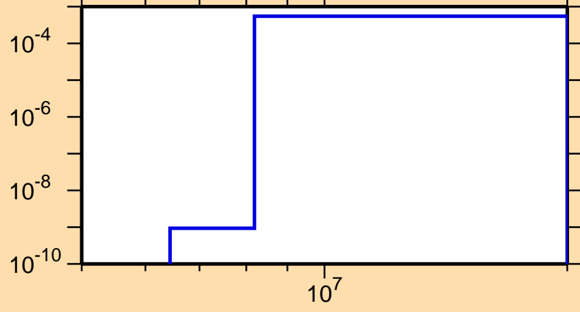
\sigma vs. E for ^{206}\text{Au}(n,p)
