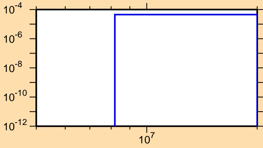
\sigma vs. E for ^{206}\text{Au}(n,t)
