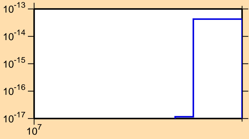
\sigma vs. E for ^{207}\text{Au}(n,3n\alpha)
