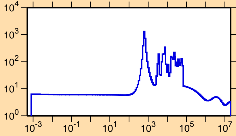
\sigma vs. E for ^{207}\text{Au}(n,\text{el.})
