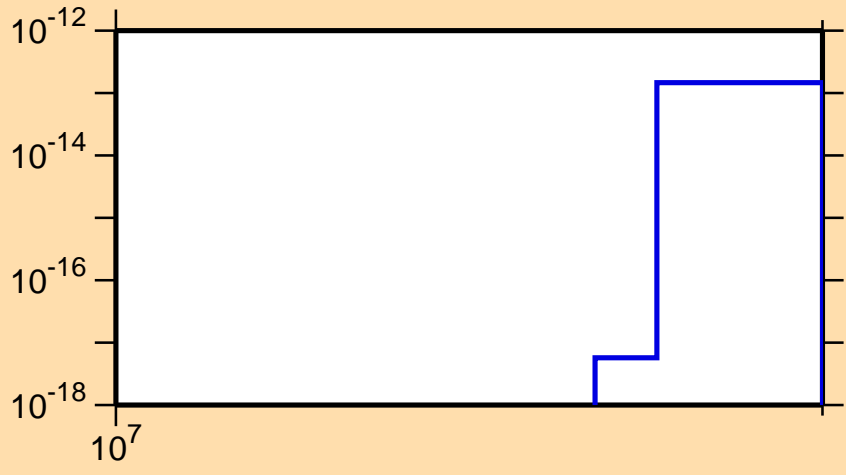
\sigma vs. E for ^{207}\text{Au}(\text{mt } 42)
