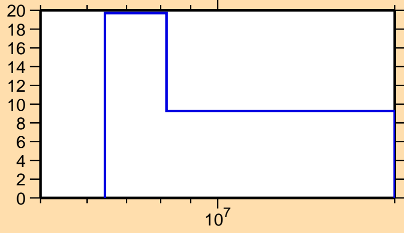
\Delta\sigma/\sigma vs. E for ^{207}\text{Au}(n,el.)
