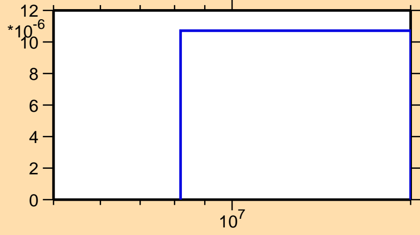
\sigma vs. E for ^{207}\text{Au}(n,d)
