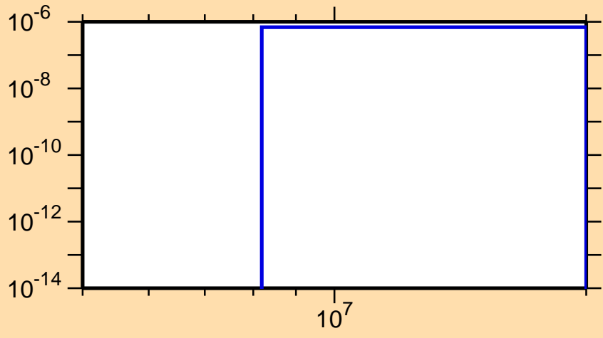
\sigma vs. E for ^{207}\text{Au}(n,nt)
