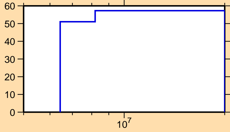
\Delta\sigma/\sigma vs. E for ^{207}\text{Au}(n,ncont.)
