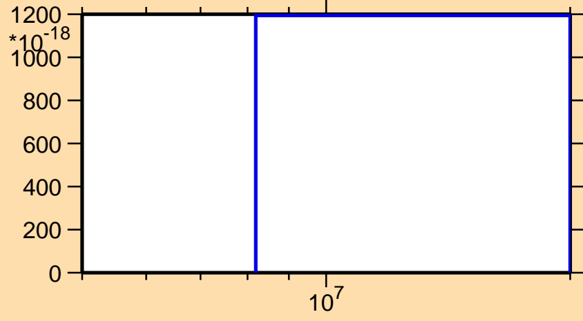
\sigma vs. E for ^{207}\text{Au}(\text{mt } 42)
