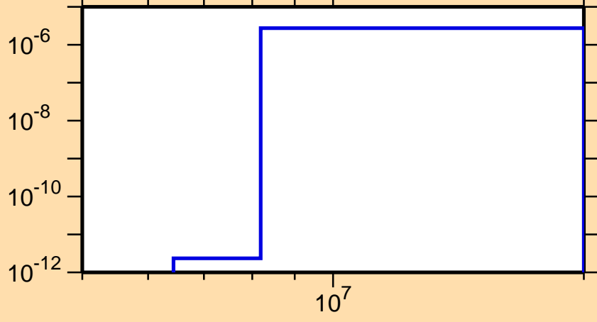
\sigma vs. E for ^{207}\text{Au}(n,n\alpha)
