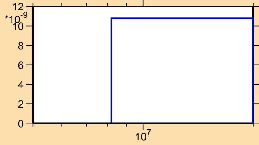
\sigma vs. E for ^{207}\text{Au}(n,\text{nd})
