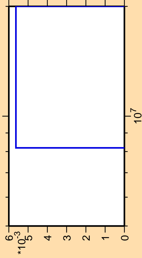
\Delta\sigma/\sigma vs. E for ^{207}\text{Au}(\text{mt } 42)
