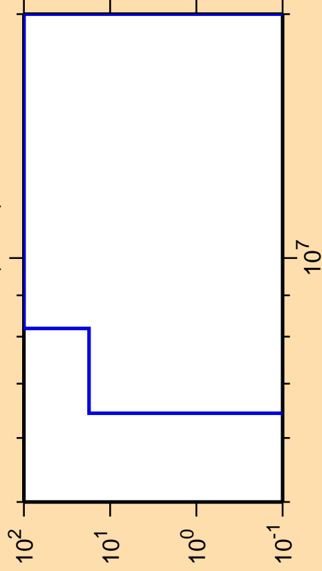
\Delta\sigma/\sigma vs. E for ^{207}\text{Au}(n,n\alpha)
