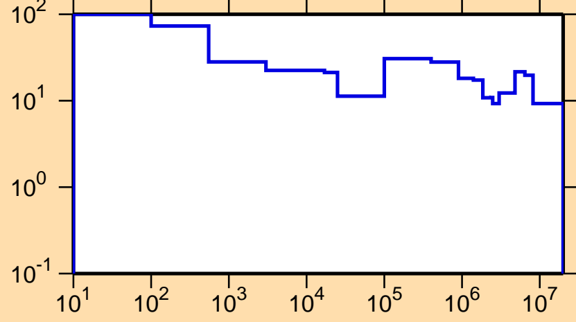
\Delta\sigma/\sigma vs. E for ^{207}\text{Au}(n,\text{el.})
