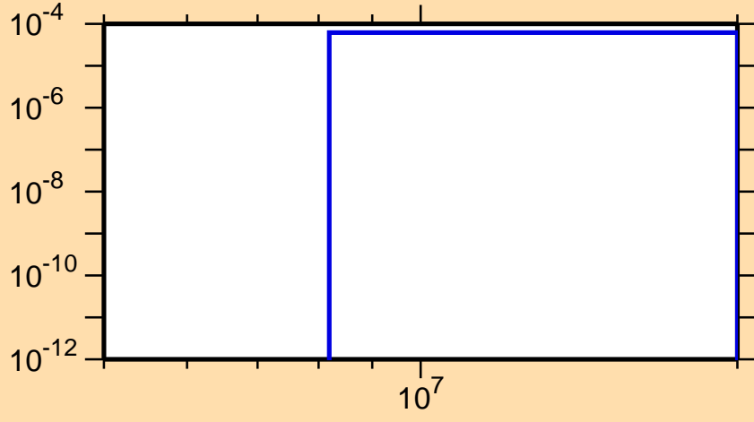
\sigma vs. E for ^{207}\text{Au}(n,p)
