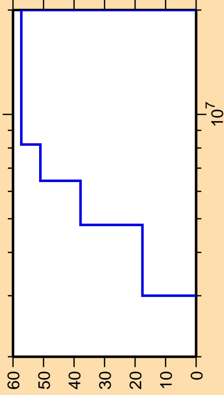
\Delta\sigma/\sigma vs. E for ^{207}\text{Au}(n,n\text{cont.})
