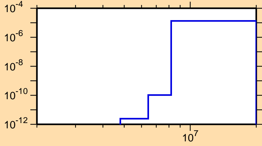
\sigma vs. E for ^{207}\text{Au}(n,\alpha)
