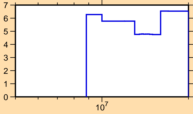
\Delta\sigma/\sigma vs. E for ^{209}\text{Au}(n,\text{tot.})
