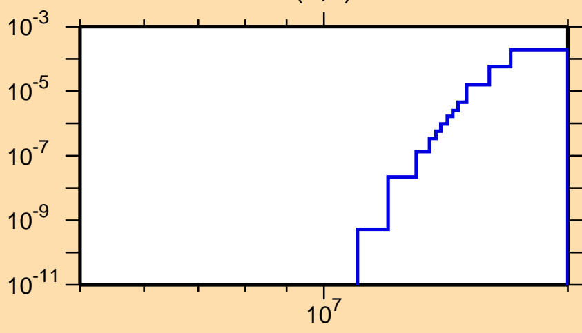
\sigma vs. E for ^{209}\text{Au}(n,d)
