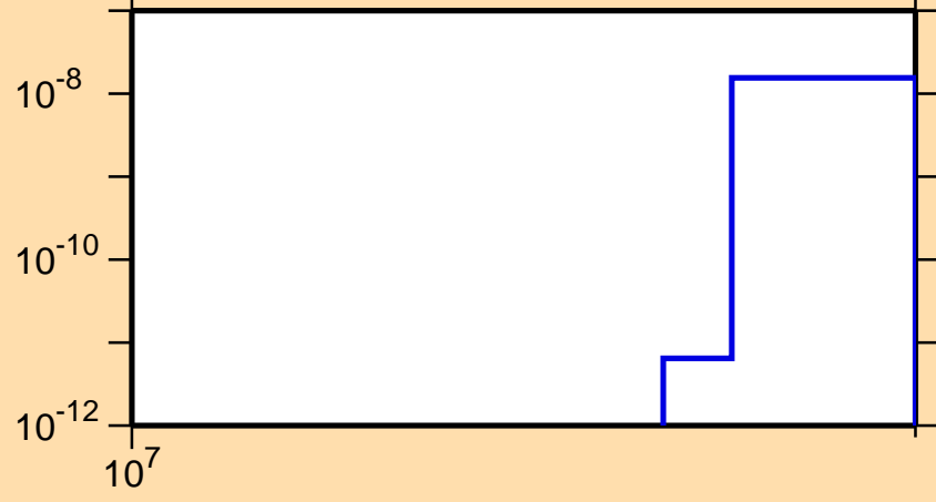
\sigma vs. E for ^{209}\text{Au}(n,2np)
