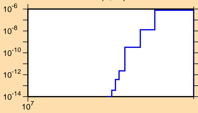
\sigma vs. E for ^{209}\text{Au}(n,\text{nd})
