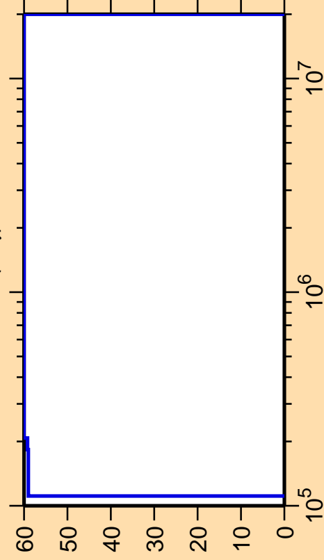
\Delta\sigma/\sigma vs. E for ^{209}\text{Au}(n,\gamma)
