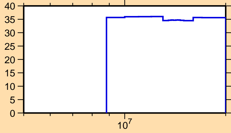
\Delta\sigma/\sigma vs. E for ^{209}\text{Au}(n,ncont.)
