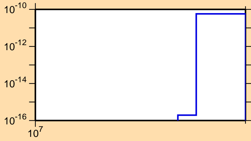
\sigma vs. E for ^{209}\text{Au}(\text{mt } 11)
