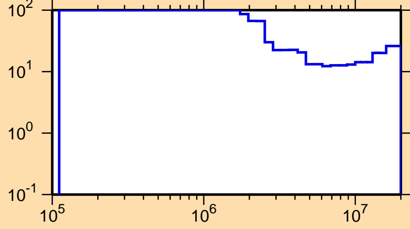
\Delta\sigma/\sigma vs. E for ^{209}\text{Au}(n,n_1)
