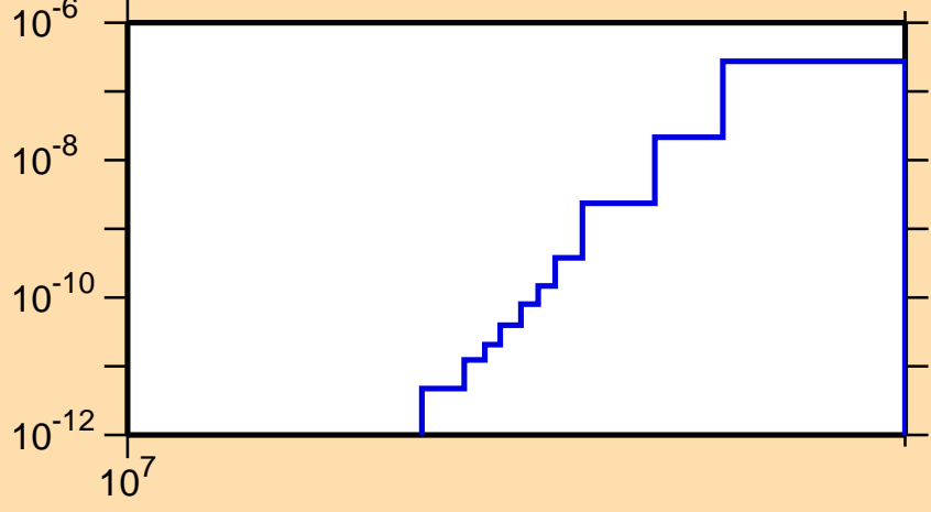
\sigma vs. E for ^{209}\text{Au}(n,2n\alpha)
