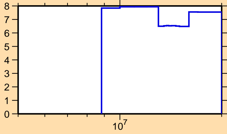
\Delta\sigma/\sigma vs. E for ^{209}\text{Au}(n,\text{nonel.})
