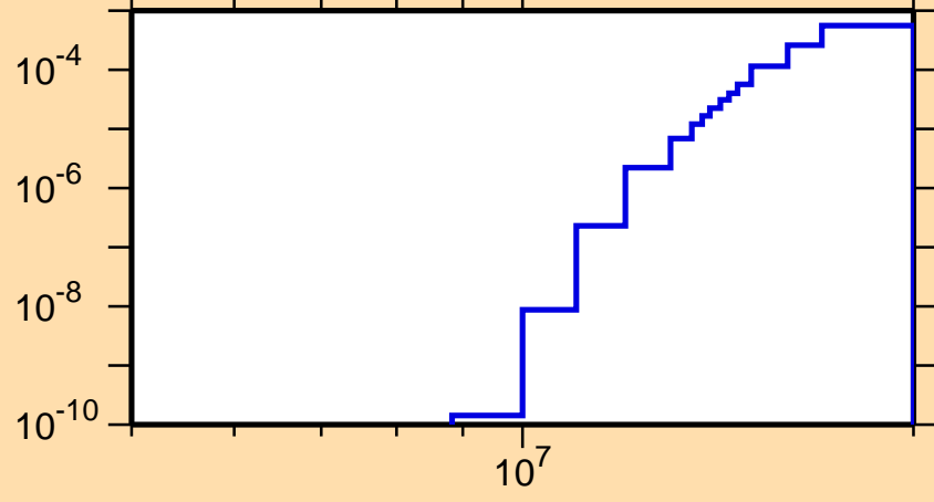
\sigma vs. E for ^{209}\text{Au}(n,p)
