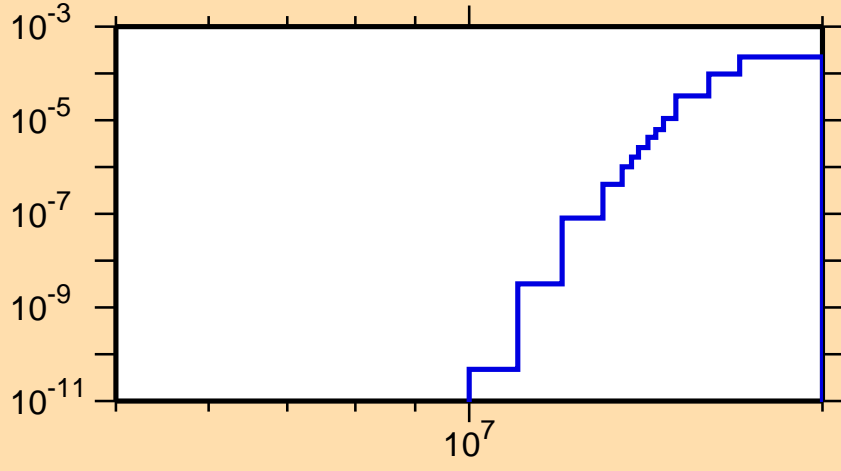
\sigma vs. E for ^{209}\text{Au}(n,t)
