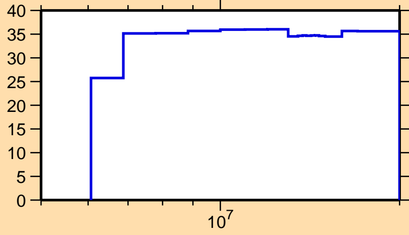
\Delta\sigma/\sigma vs. E for ^{209}\text{Au}(n,n\text{cont.})
