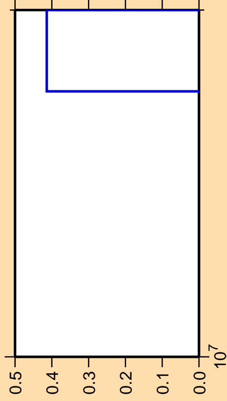
\Delta\sigma/\sigma vs. E for ^{209}\text{Au}(\text{mt } 42)
