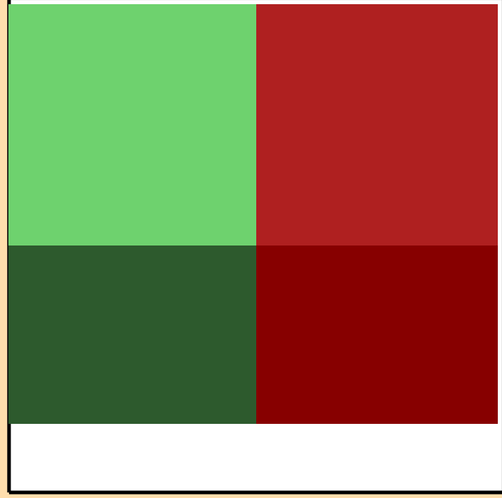
\Delta\sigma/\sigma vs. E for ^{209}\text{Au}(n,n_1)
