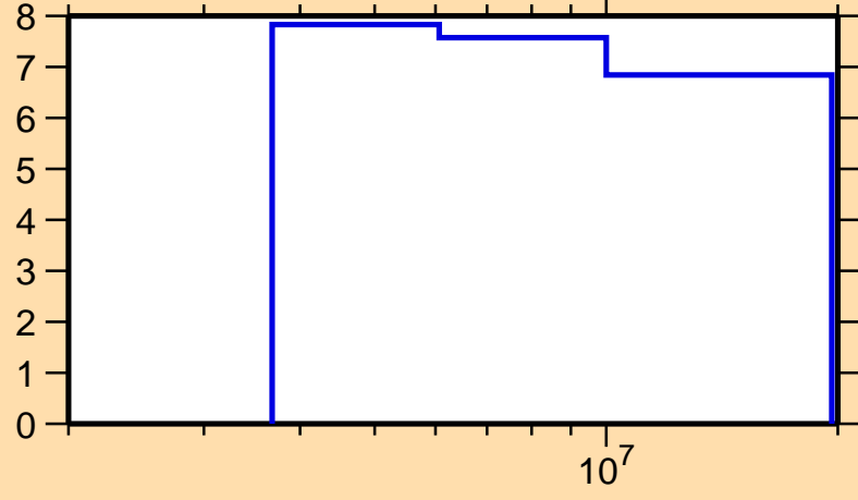
\Delta\sigma/\sigma vs. E for ^{209}\text{Au}(n,\text{nonel.})
