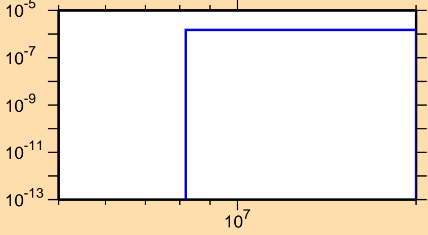
\sigma vs. E for ^{209}\text{Au}(n,nt)
