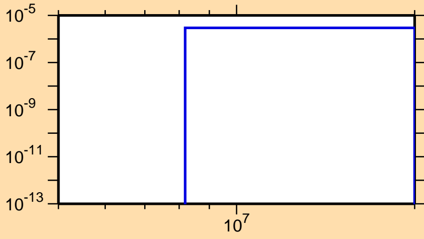
\sigma vs. E for ^{209}\text{Au}(n,n\alpha)
