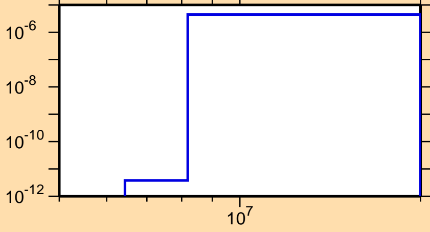
\sigma vs. E for ^{209}\text{Au}(n,\alpha)
