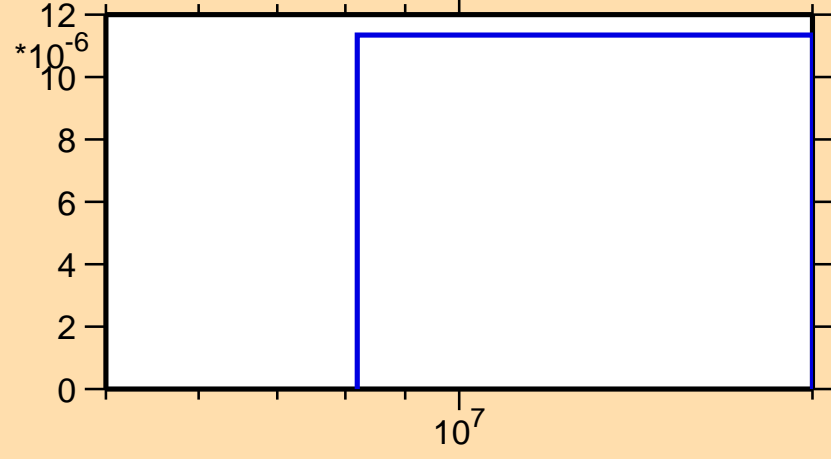
\sigma vs. E for ^{209}\text{Au}(n,t)
