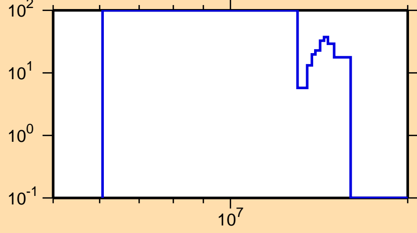
\Delta\sigma/\sigma vs. E for ^{210}\text{Au}(n,n_1)
