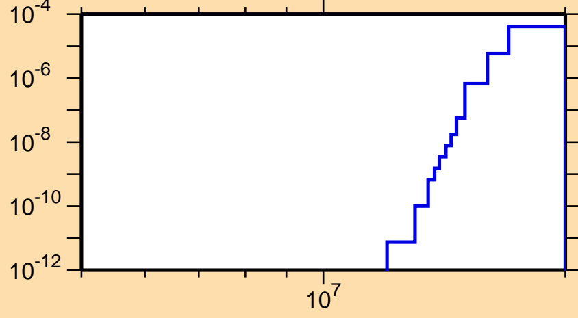
\sigma vs. E for ^{210}\text{Au}(n,\text{nt})
