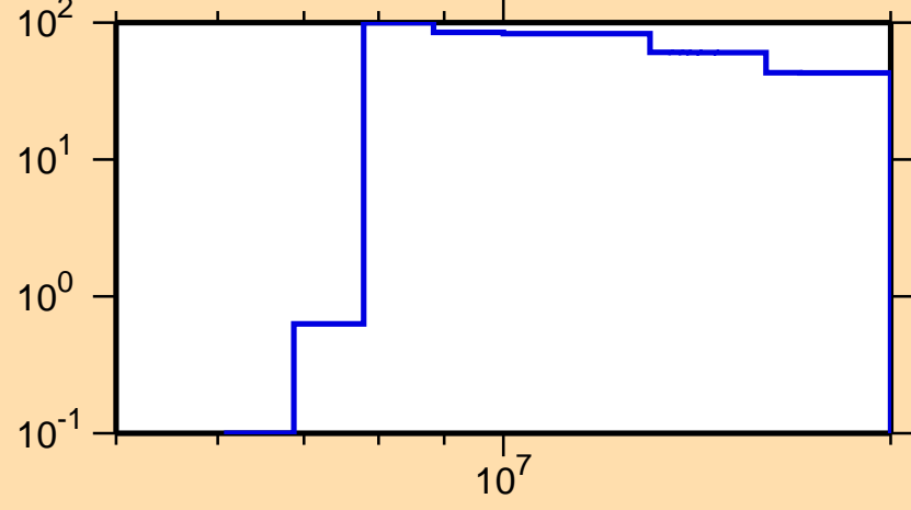
\Delta\sigma/\sigma vs. E for ^{210}\text{Au}(n,p)
