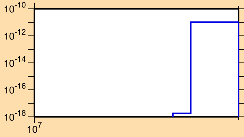
\sigma vs. E for ^{210}\text{Au}(\text{mt } 11)
