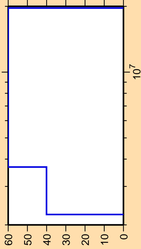
\Delta\sigma/\sigma vs. E for ^{210}\text{Au}(n,n\text{cont.})
