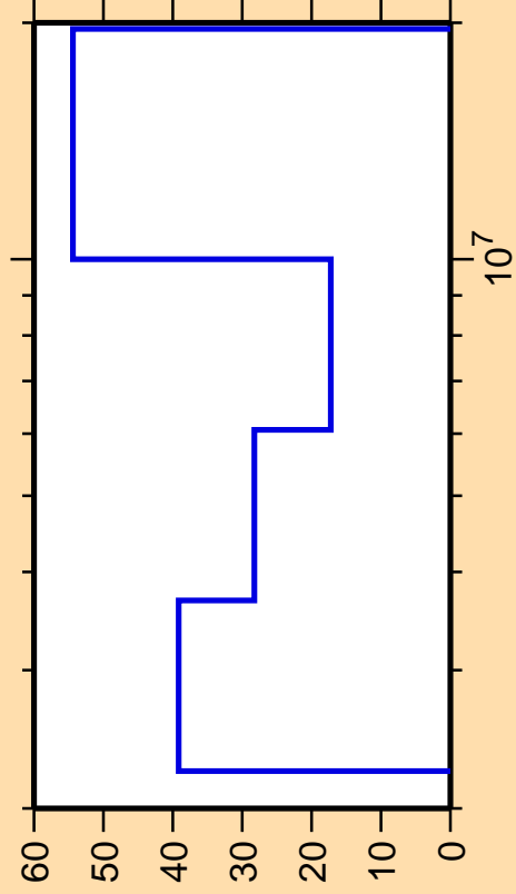
\Delta\sigma/\sigma vs. E for ^{210}\text{Au}(n,2n)
