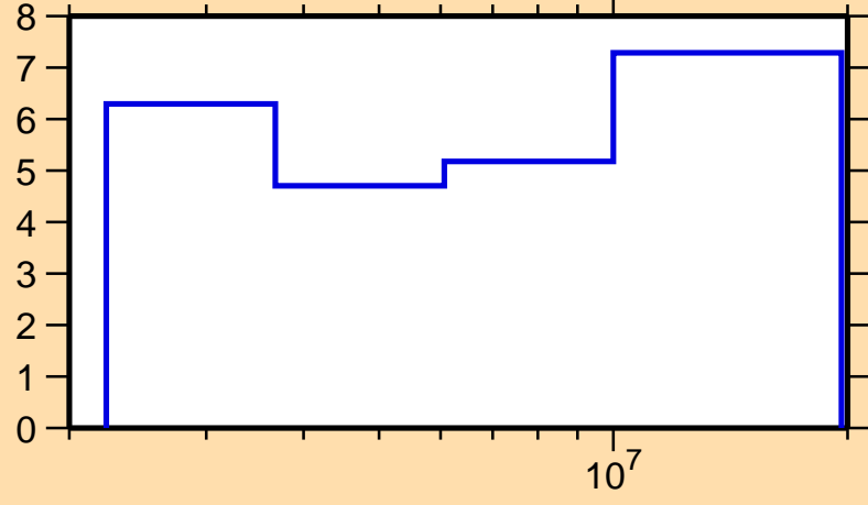
\Delta\sigma/\sigma vs. E for ^{210}\text{Au}(n,\text{nonel.})
