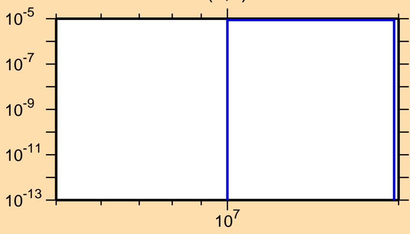
\sigma vs. E for ^{210}\text{Au}(n,d)
