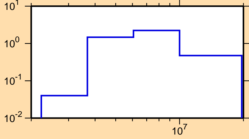
\sigma vs. E for ^{210}\text{Au}(n,2n)
