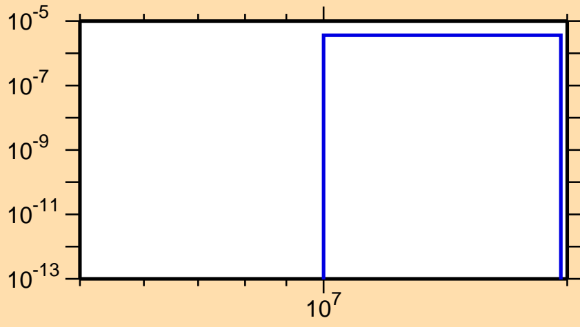
\sigma vs. E for ^{210}\text{Au}(n,np)
