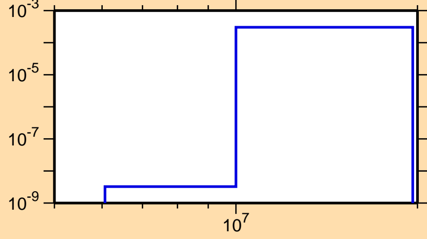
\sigma vs. E for ^{210}\text{Au}(n,p)
