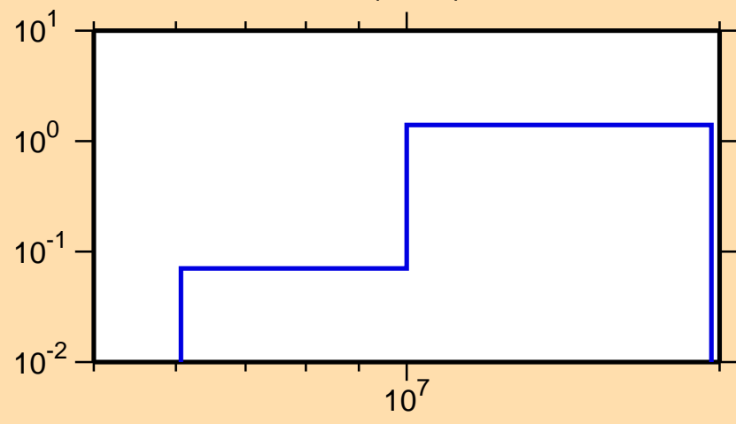
\sigma vs. E for ^{210}\text{Au}(n,3n)
