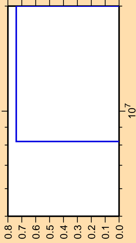
\Delta\sigma/\sigma vs. E for ^{210}\text{Au}(\text{mt } 11)
