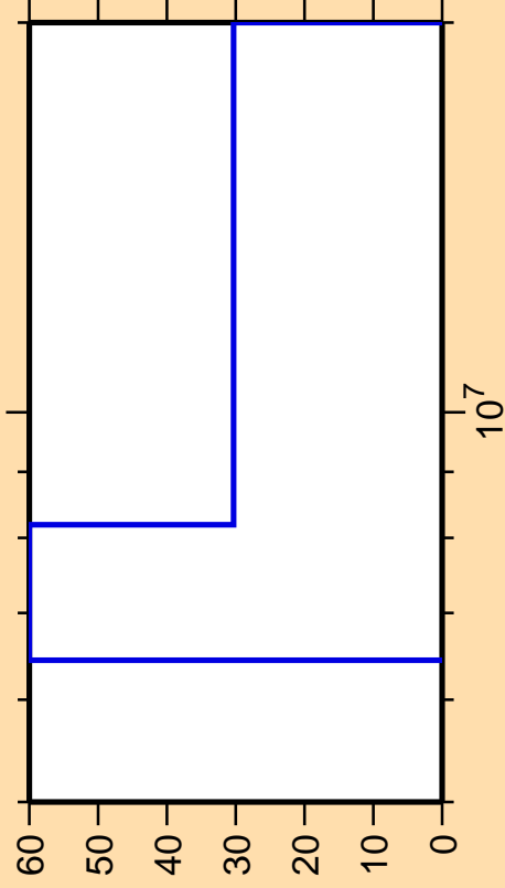
\Delta\sigma/\sigma vs. E for ^{210}\text{Au}(n,3n)
