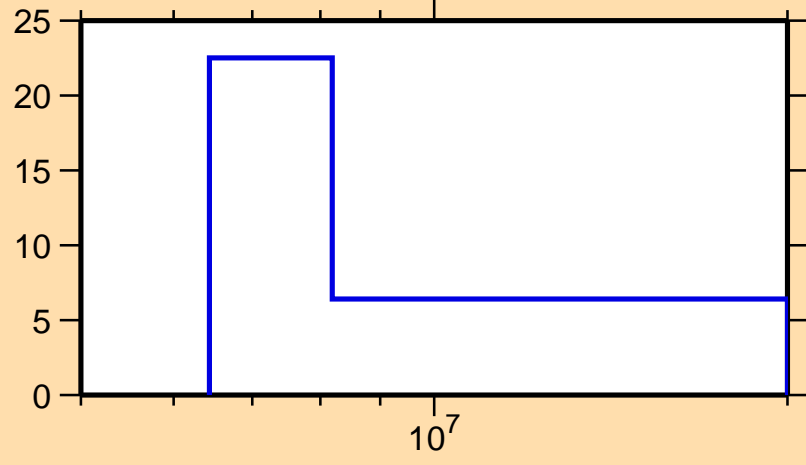
\Delta\sigma/\sigma vs. E for ^{210}\text{Au}(n,el.)
