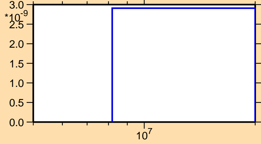
\sigma vs. E for ^{210}\text{Au}(n,2np)
