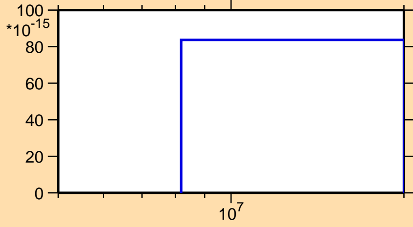
\sigma vs. E for ^{210}\text{Au}(\text{mt } 11)
