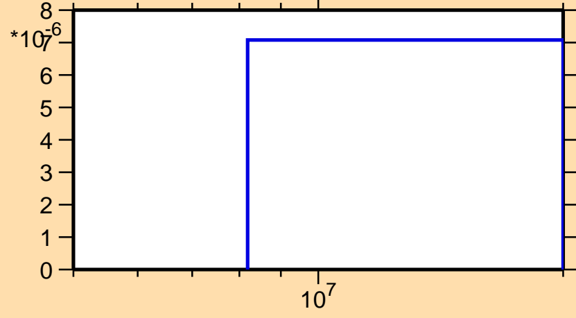
\sigma vs. E for ^{210}\text{Au}(n,d)
