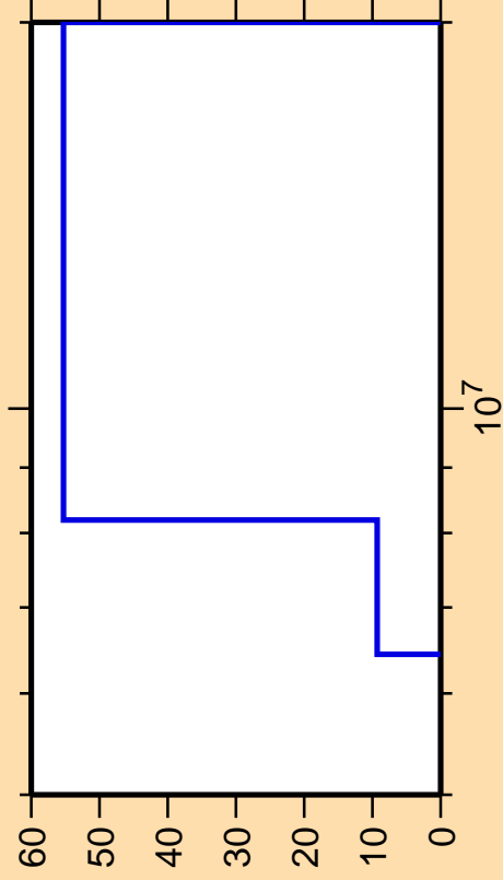
\Delta\sigma/\sigma vs. E for ^{210}\text{Au}(n,p)
