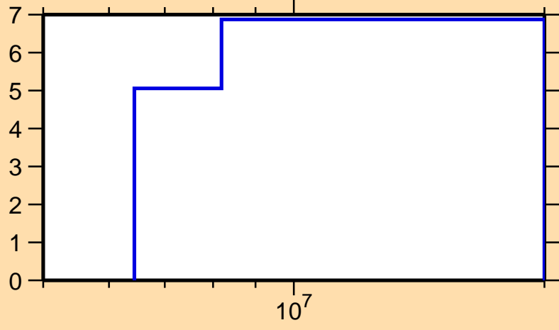
\Delta\sigma/\sigma vs. E for ^{210}\text{Au}(n,\text{nonel.})
