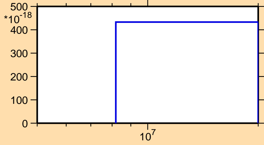
\sigma vs. E for ^{210}\text{Au}(\text{mt } 42)
