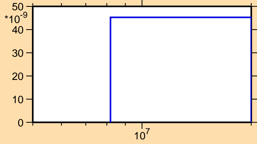
\sigma vs. E for ^{210}\text{Au}(n,\text{nd})
