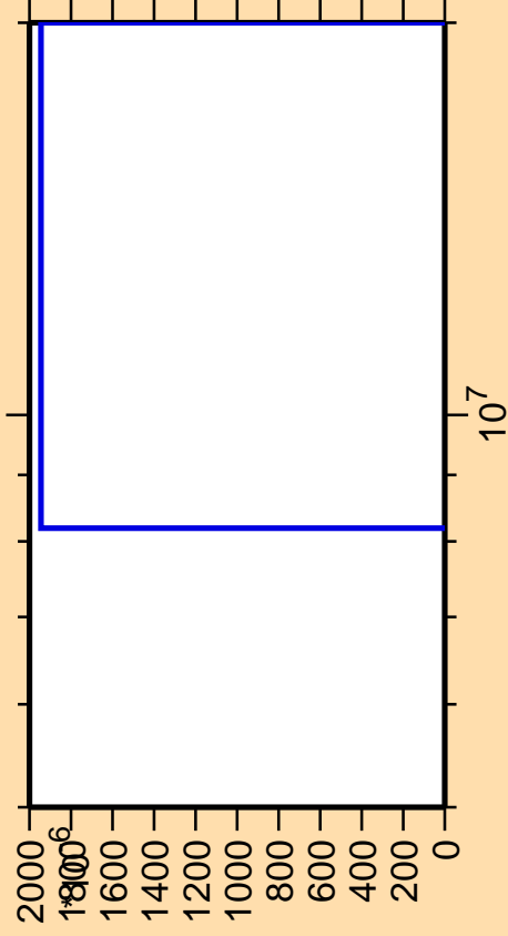
\Delta\sigma/\sigma vs. E for ^{210}\text{Au}(\text{mt } 42)
