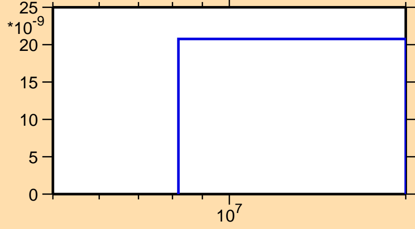
\sigma vs. E for ^{210}\text{Au}(n,2n\alpha)
