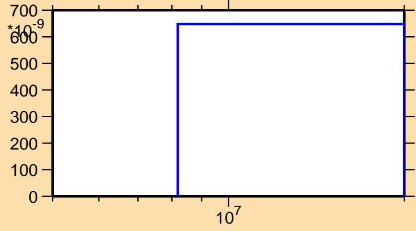
\sigma vs. E for ^{210}\text{Au}(n,nt)
