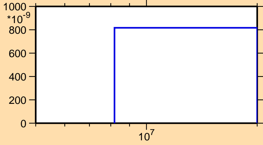
\sigma vs. E for ^{210}\text{Au}(n,n\alpha)
