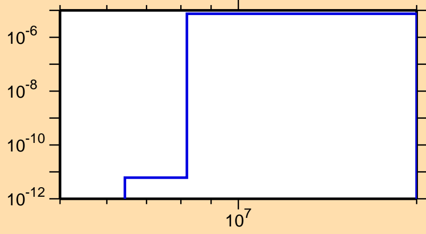
\sigma vs. E for ^{210}\text{Au}(n,\alpha)
