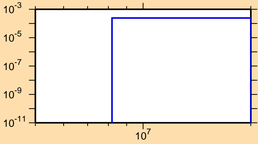
\sigma vs. E for ^{210}\text{Au}(n,p)
