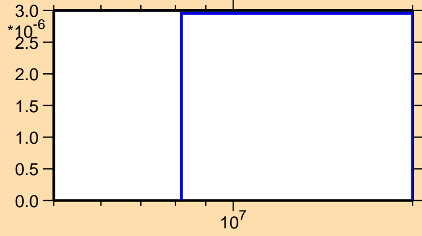
\sigma vs. E for ^{210}\text{Au}(n,np)
