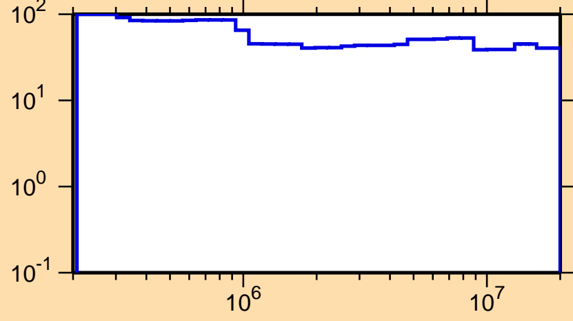
\Delta\sigma/\sigma vs. E for ^{116}\text{Ba}(n,n_1)
