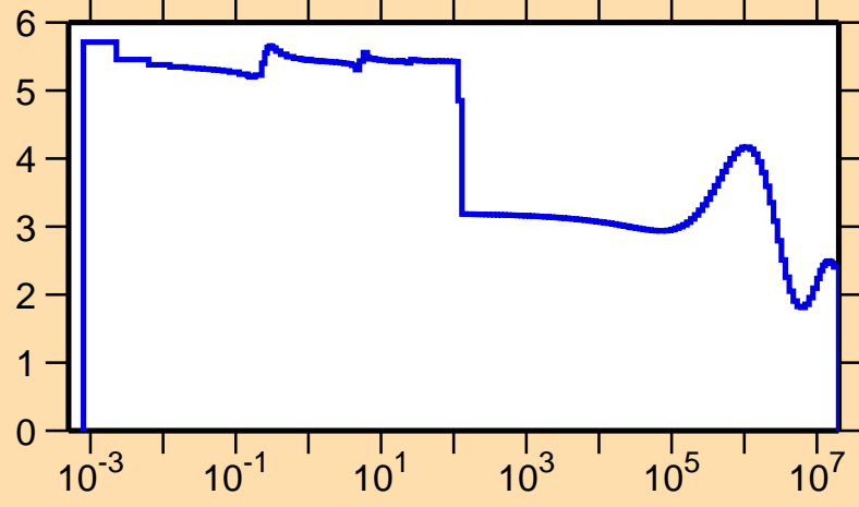
\sigma vs. E for ^{116}\text{Ba}(n,\text{el.})
