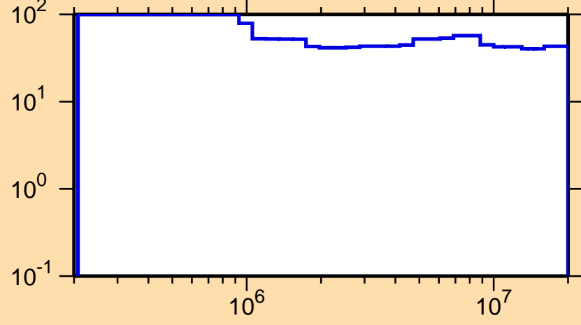
\Delta\sigma/\sigma vs. E for ^{116}\text{Ba}(n,\text{inel.})
