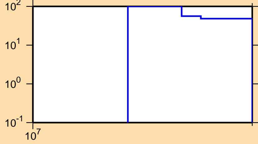
\Delta\sigma/\sigma vs. E for ^{116}\text{Ba}(n,2n)
