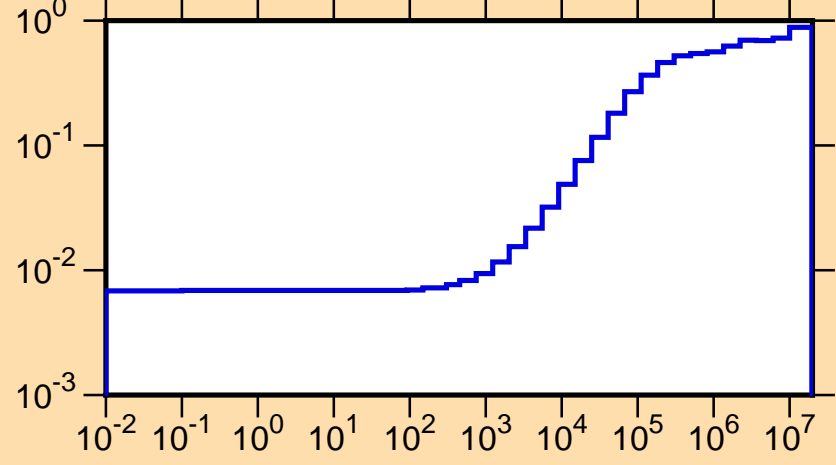
\mu vs. E for ^{116}\text{Ba}(\text{mt251})
