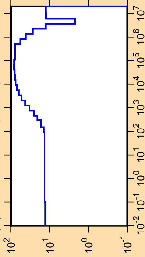
\Delta\mu/\mu vs. E for ^{116}\text{Ba}(\text{mt251})
