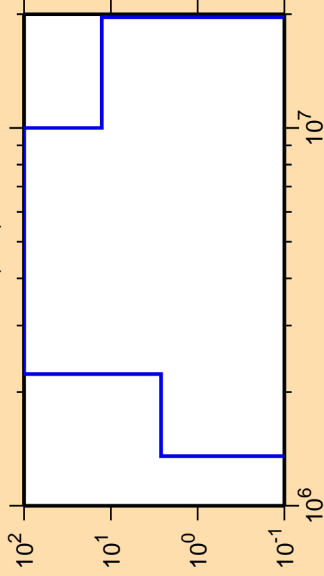
\Delta\sigma/\sigma vs. E for ^{116}\text{Ba}(n,d)
