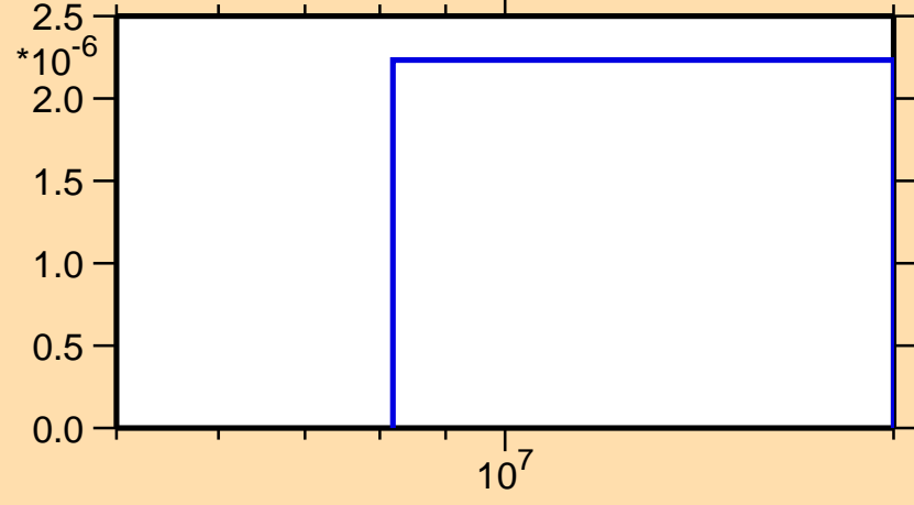
\sigma vs. E for ^{116}\text{Ba}(n,2n)
