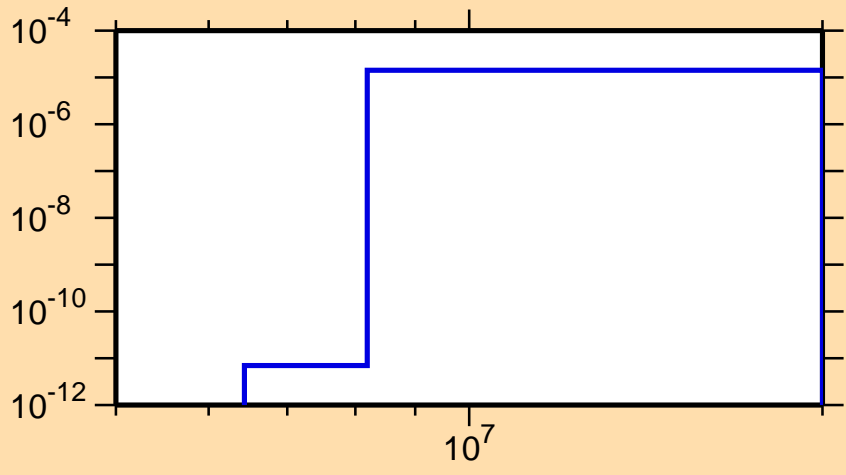
\sigma vs. E for ^{116}\text{Ba}(\text{mt } 45)
