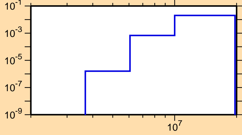
\sigma vs. E for ^{117}\text{Ba}(n,d)
