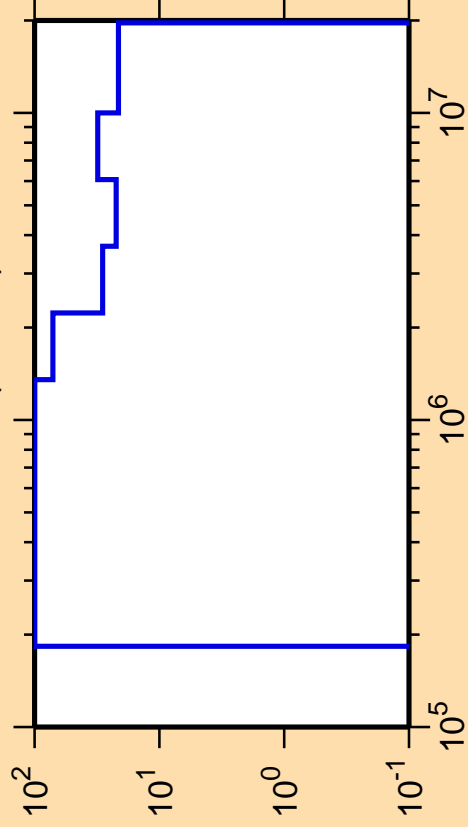
\Delta\sigma/\sigma vs. E for ^{117}\text{Ba}(n,\text{inel.})
