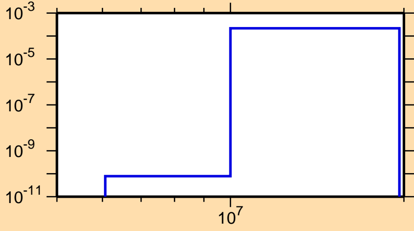
\sigma vs. E for ^{117}\text{Ba}(n,t)
