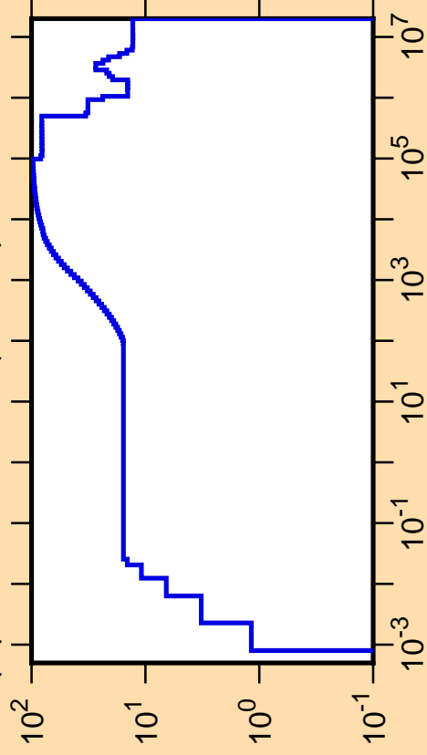
\Delta\mu/\mu vs. E for ^{118}\text{Ba}(\text{mt251})
