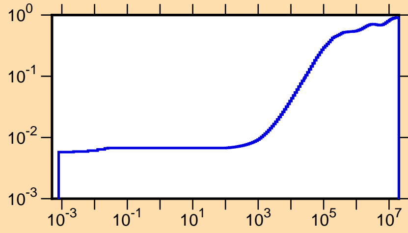
\mu vs. E for ^{118}\text{Ba}(\text{mt251})
