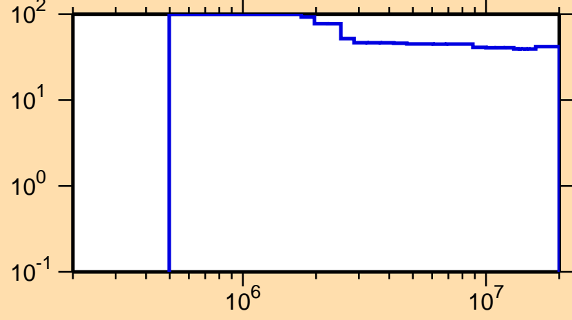
\Delta\sigma/\sigma vs. E for ^{118}\text{Ba}(n,\text{inel.})
