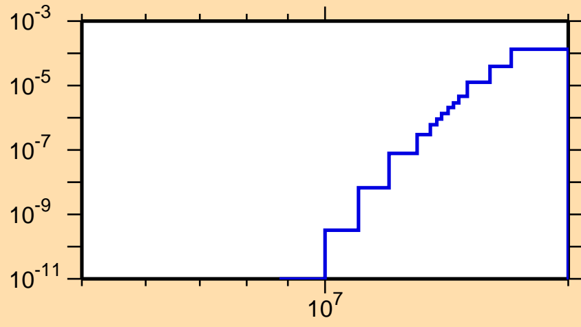
\sigma vs. E for ^{118}\text{Ba} (mt 45)
