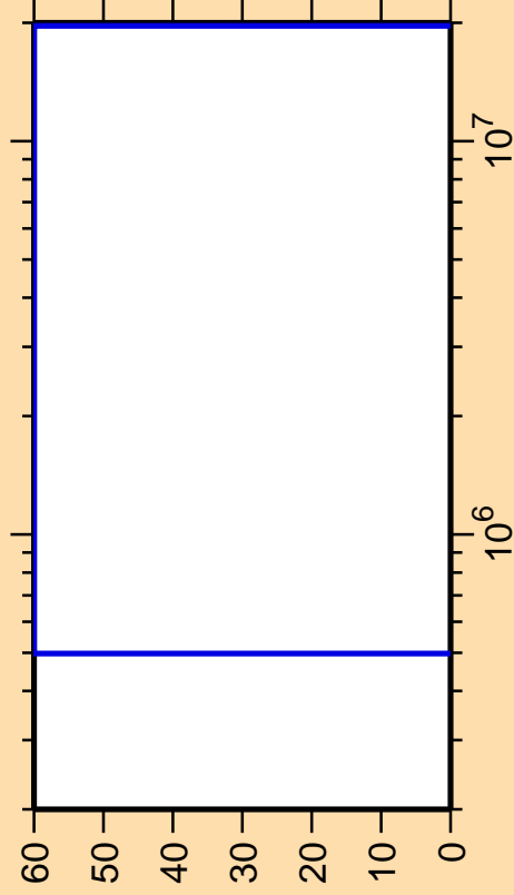
\Delta\sigma/\sigma vs. E for ^{118}\text{Ba}(n,\text{ncont.})
