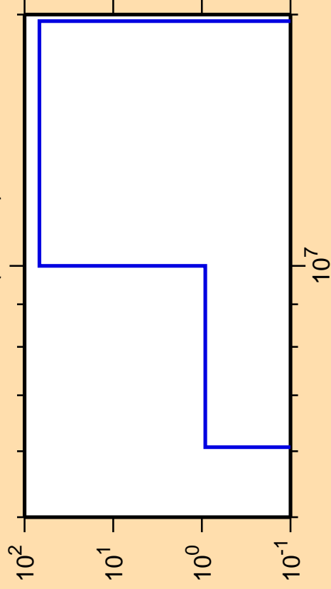
\Delta\sigma/\sigma vs. E for ^{118}\text{Ba} (mt 45)
