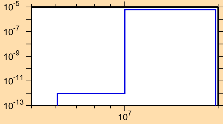
\sigma vs. E for ^{118}\text{Ba} (mt 45)
