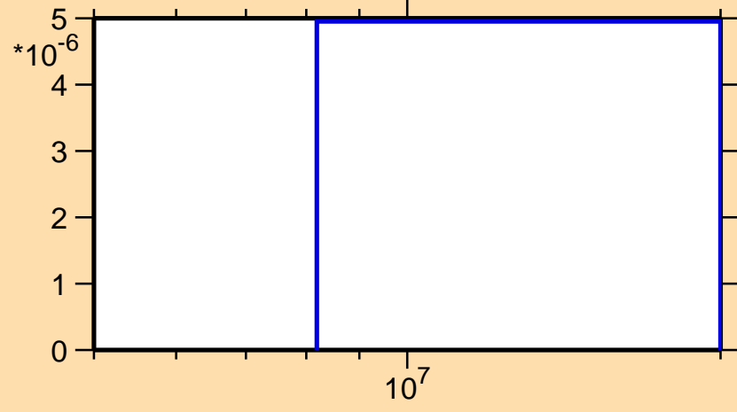
\sigma vs. E for ^{118}\text{Ba}(\text{mt } 45)
