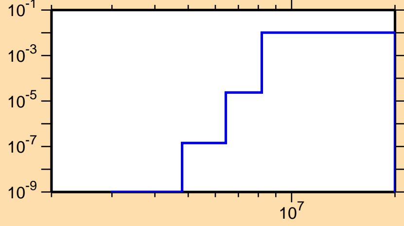
\sigma vs. E for ^{118}\text{Ba}(n,d)
