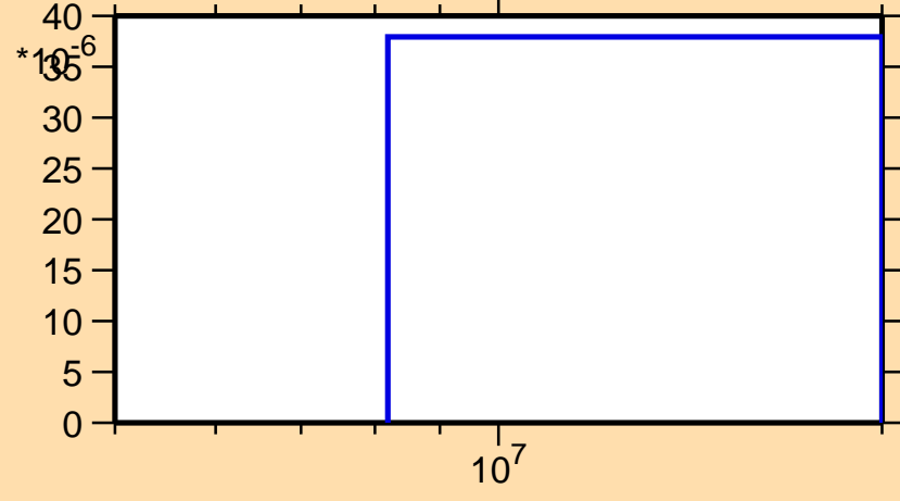
\sigma vs. E for ^{118}\text{Ba}(n,2n)
