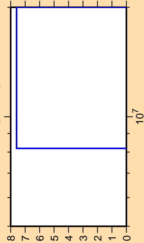
\Delta\sigma/\sigma vs. E for ^{118}\text{Ba}(n,2n\alpha)
