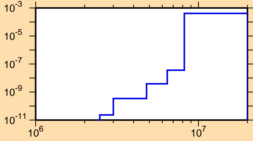
\sigma vs. E for ^{118}\text{Ba}(n,\text{He3})
