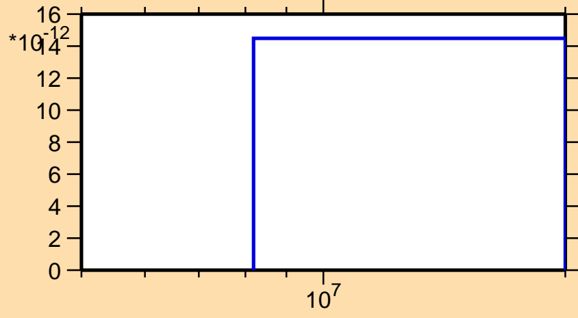
\sigma vs. E for ^{118}\text{Ba}(\text{mt } 34)
