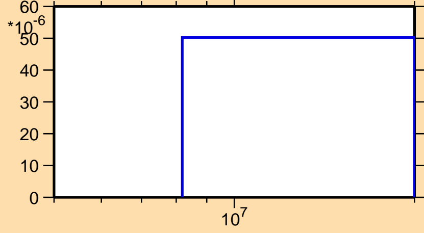
\sigma vs. E for ^{118}\text{Ba}(n,t)
