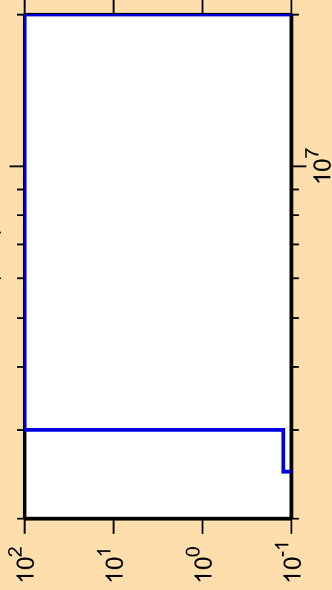
\Delta\sigma/\sigma vs. E for ^{118}\text{Ba}(n,d)
