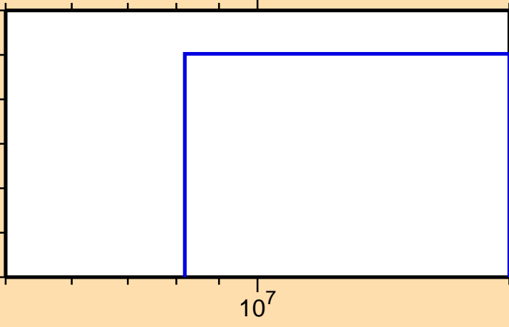
\sigma vs. E for ^{118}\text{Ba}(n,t)
