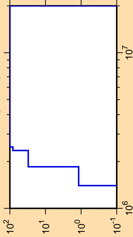
\Delta\sigma/\sigma vs. E for ^{118}\text{Ba}(n,\text{He3})
