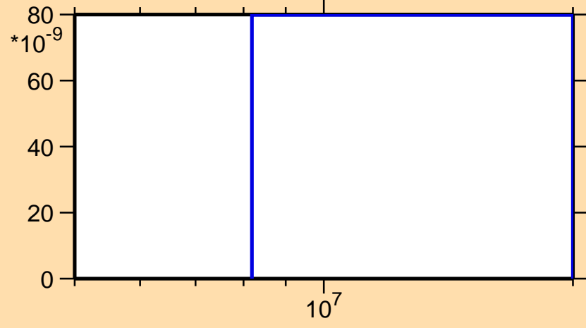
\sigma vs. E for ^{118}\text{Ba}(\text{mt117})
