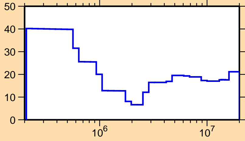
\Delta\sigma/\sigma vs. E for ^{119}\text{Ba}(n,n\text{nonel.})
