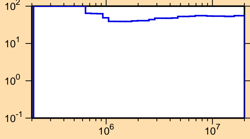
\Delta\sigma/\sigma vs. E for ^{119}\text{Ba}(n,\text{inel.})
