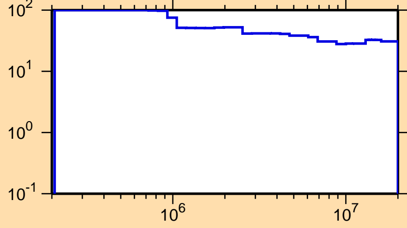
\Delta\sigma/\sigma vs. E for ^{119}\text{Ba}(n,n_1)
