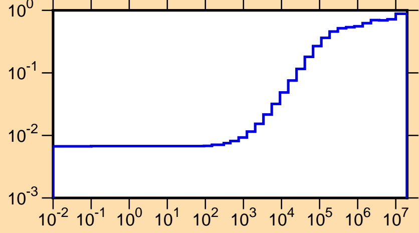
\mu vs. E for ^{119}\text{Ba}(\text{mt251})
