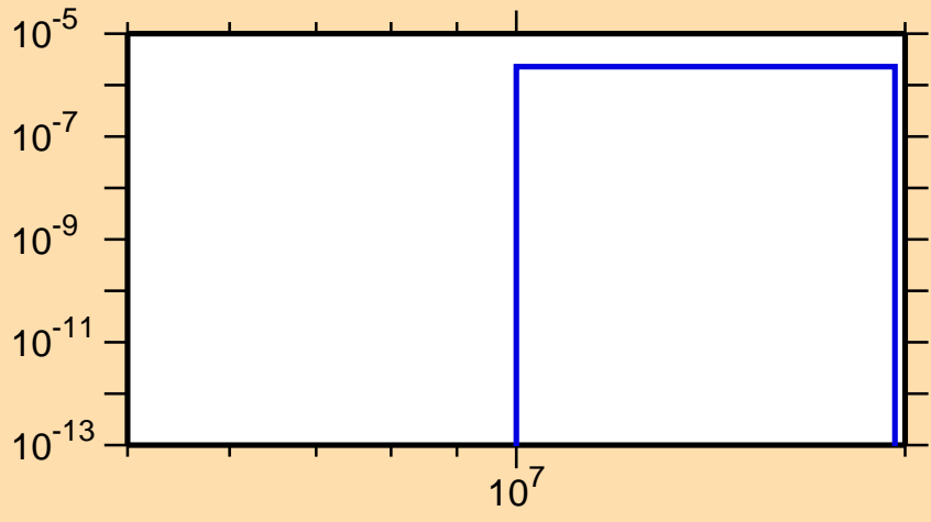
\sigma vs. E for ^{119}\text{Ba}(\text{mt } 45)
