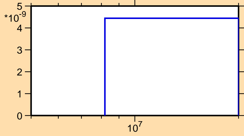
\sigma vs. E for ^{119}\text{Ba}(\text{mt } 34)
