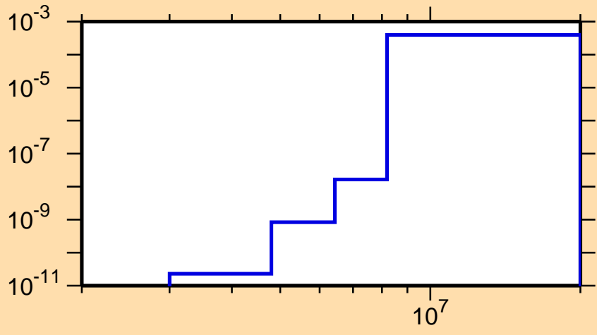
\sigma vs. E for ^{119}\text{Ba}(n,\text{He3})
