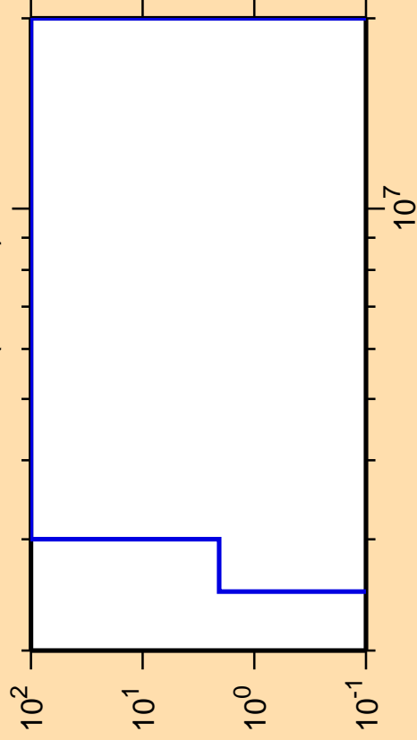
\Delta\sigma/\sigma vs. E for ^{119}\text{Ba}(n,\text{He3})
