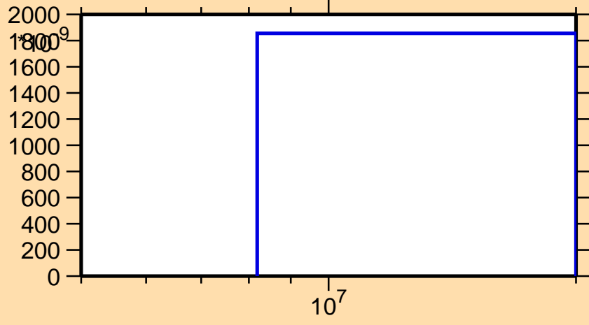
\sigma vs. E for ^{119}\text{Ba}(\text{mt } 45)
