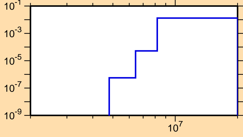
\sigma vs. E for ^{119}\text{Ba}(n,d)
