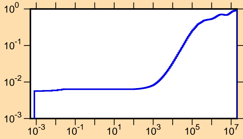
\mu vs. E for ^{120}\text{Ba}(\text{mt251})
