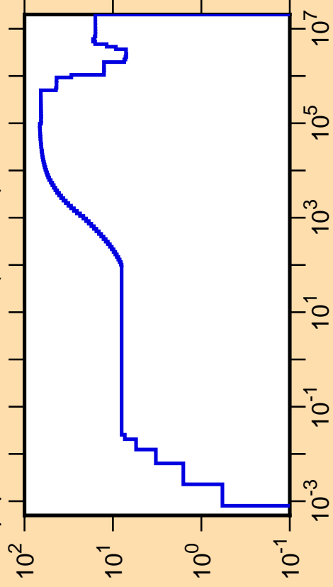
\Delta\mu/\mu vs. E for ^{120}\text{Ba}(\text{mt251})
