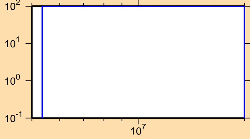
\Delta\sigma/\sigma vs. E for ^{120}\text{Ba}(n,n\text{cont.})
