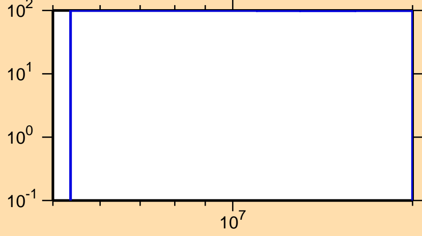
\Delta\sigma/\sigma vs. E for ^{120}\text{Ba}(n,ncont.)
