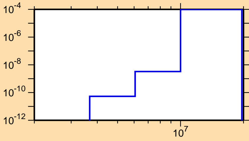
\sigma vs. E for ^{120}\text{Ba}(n,\text{He3})
