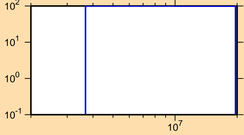
\Delta\sigma/\sigma vs. E for ^{120}\text{Ba}(n,ncont.)
