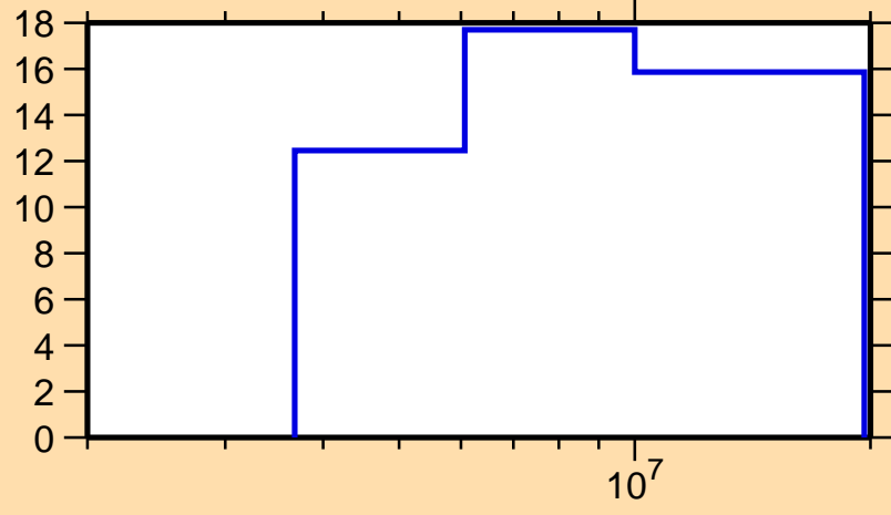
\Delta\sigma/\sigma vs. E for ^{120}\text{Ba}(n,n\text{onel.})
