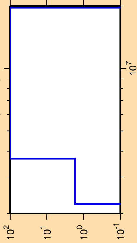
\Delta\sigma/\sigma vs. E for ^{120}\text{Ba}(n,\text{He3})
