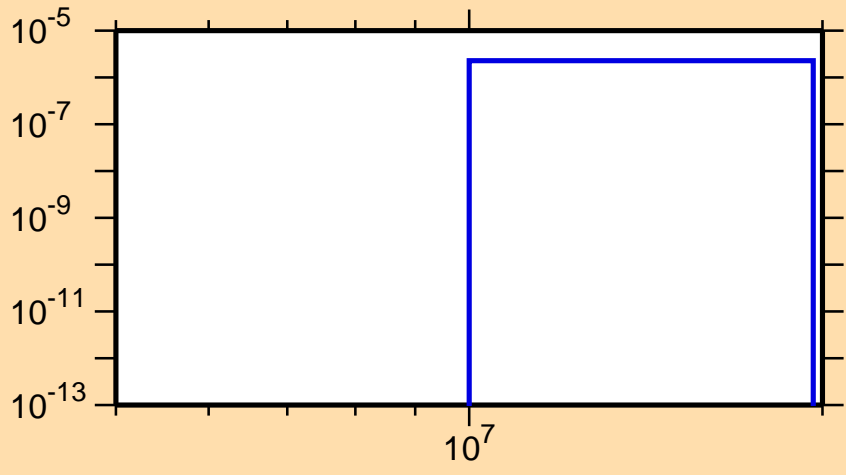
\sigma vs. E for ^{120}\text{Ba} (mt 45)
