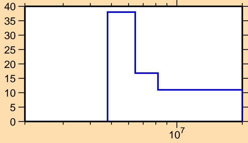
\Delta\sigma/\sigma vs. E for ^{120}\text{Ba}(n,el.)
