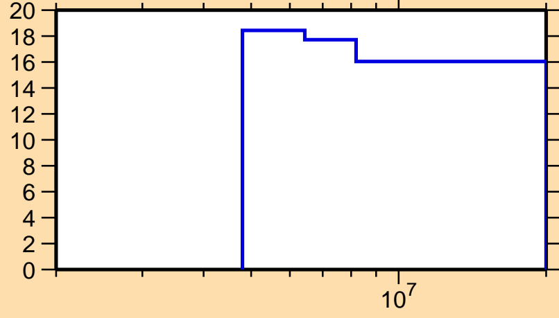
\Delta\sigma/\sigma vs. E for ^{120}\text{Ba}(n,n\text{nonel.})
