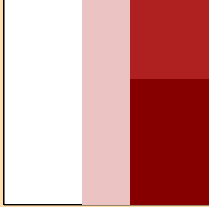
\Delta\sigma/\sigma vs. E for ^{120}\text{Ba}(n,ncont.)
