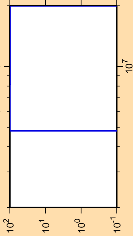
\Delta\sigma/\sigma vs. E for ^{120}\text{Ba}(n,ncont.)
