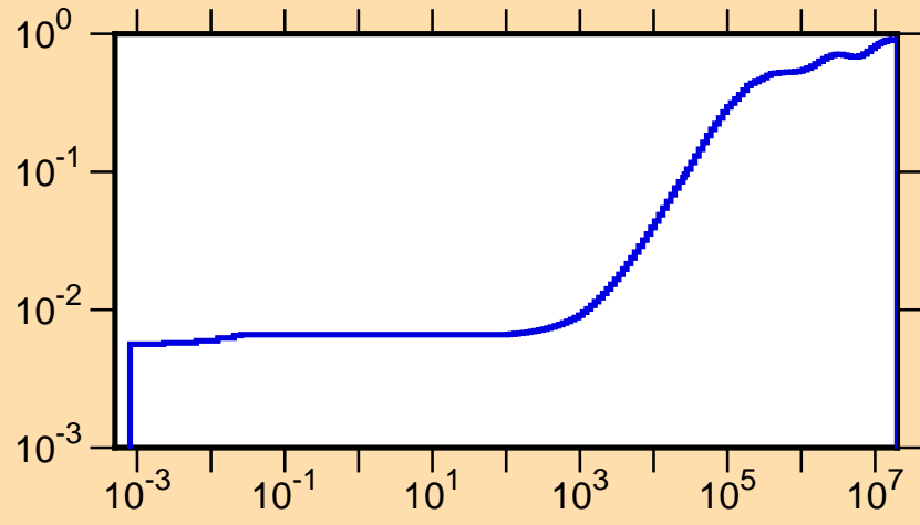
\mu vs. E for ^{121}\text{Ba}(\text{mt251})
