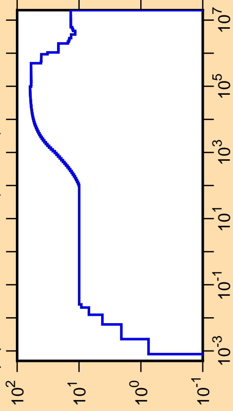
\Delta\mu/\mu vs. E for ^{121}\text{Ba}(\text{mt251})
