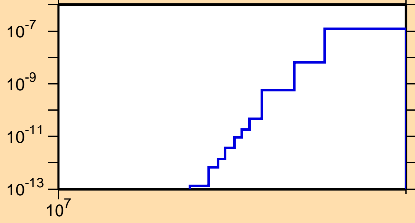
\sigma vs. E for ^{121}\text{Ba} (mt 34)
