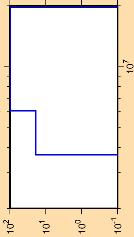
\Delta\sigma/\sigma vs. E for ^{121}\text{Ba}(n,\text{He3})
