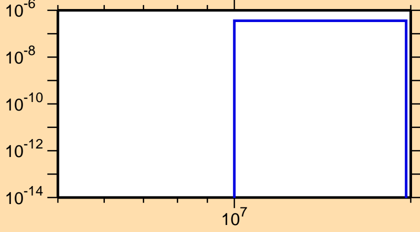
\sigma vs. E for ^{121}\text{Ba}(\text{mt } 45)
