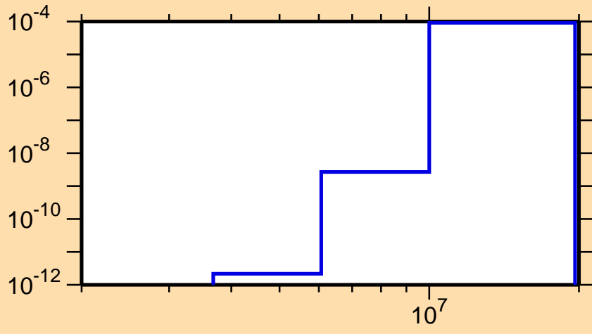
\sigma vs. E for ^{121}\text{Ba}(n,\text{He3})
