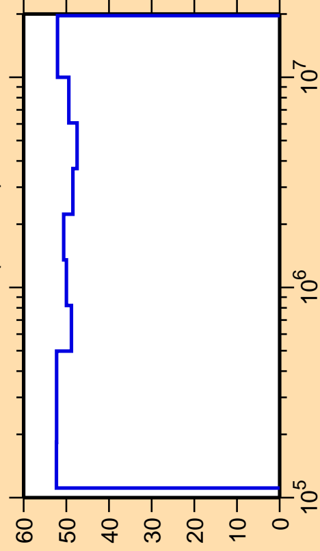
\Delta\sigma/\sigma vs. E for ^{121}\text{Ba}(n,\text{inel.})
