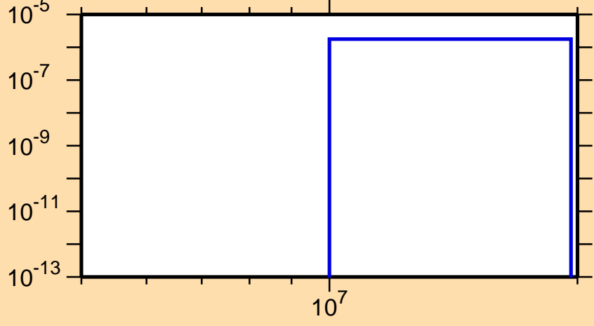
\sigma vs. E for ^{121}\text{Ba}(n,\text{pt})
