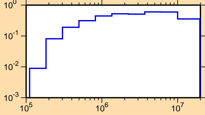
\sigma vs. E for ^{121}\text{Ba}(n,\text{inel.})
