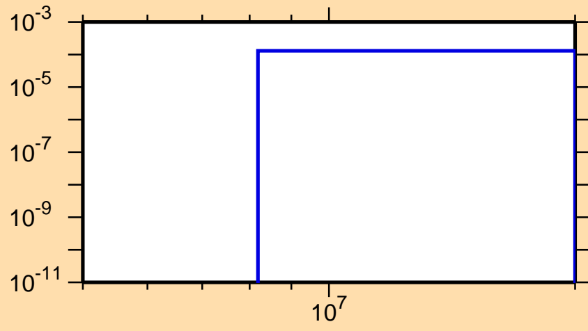
\sigma vs. E for ^{121}\text{Ba}(n,t)
