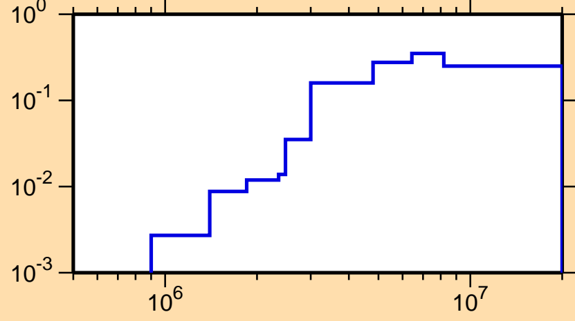
\sigma vs. E for ^{121}\text{Ba}(n,n\text{cont.})
