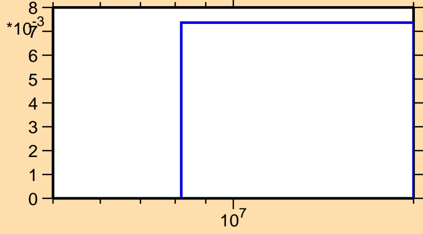
\sigma vs. E for ^{121}\text{Ba}(n,2n)
