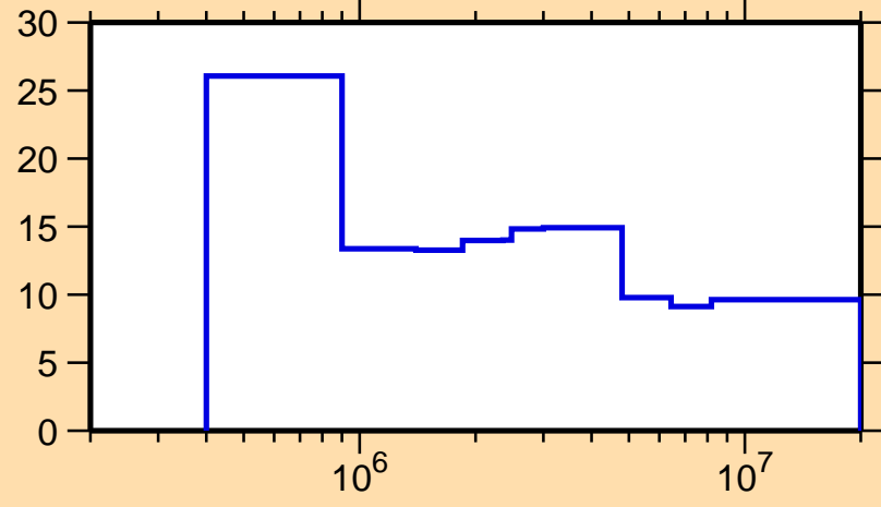
\Delta\sigma/\sigma vs. E for ^{121}\text{Ba}(n,n\text{nonel.})
