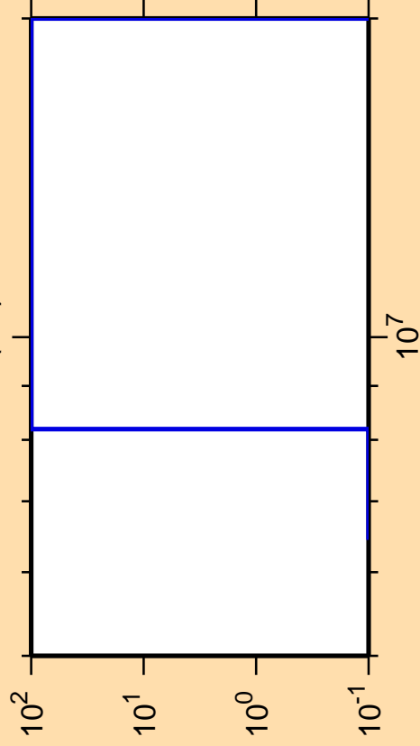
\Delta\sigma/\sigma vs. E for ^{121}\text{Ba}(n,t)
