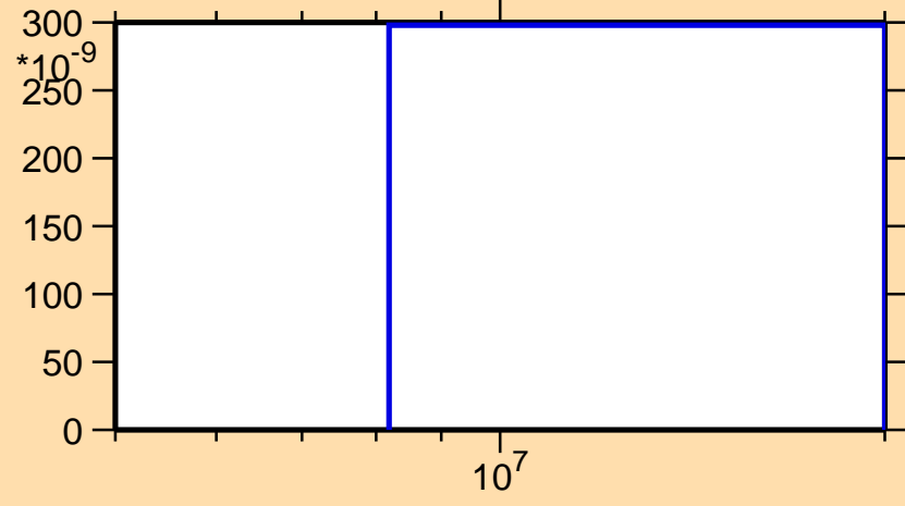
\sigma vs. E for ^{121}\text{Ba} (mt 45)
