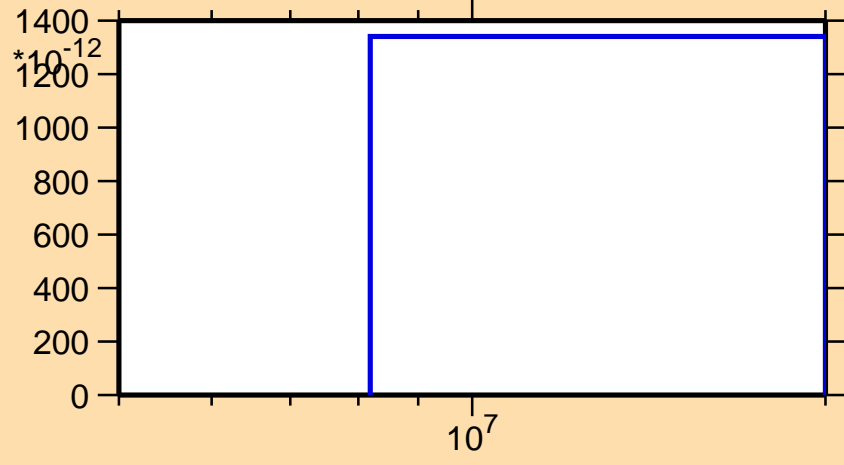
\sigma vs. E for ^{121}\text{Ba}(\text{mt } 34)
