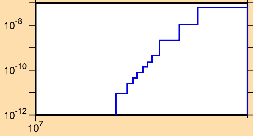
\sigma vs. E for ^{122}\text{Ba}(\text{mt117})
