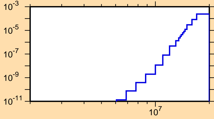
\sigma vs. E for ^{122}\text{Ba}(n,\text{He3})
