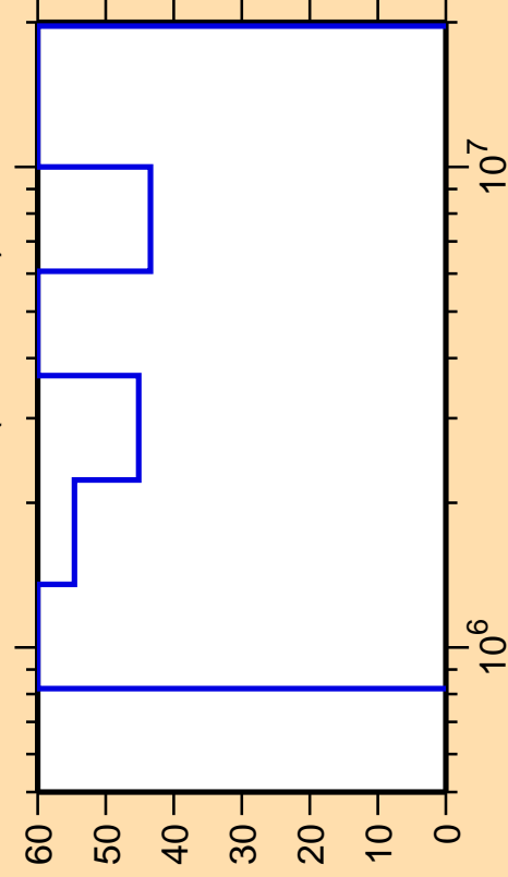
\Delta\sigma/\sigma vs. E for ^{122}\text{Ba}(n,\text{ncont.})
