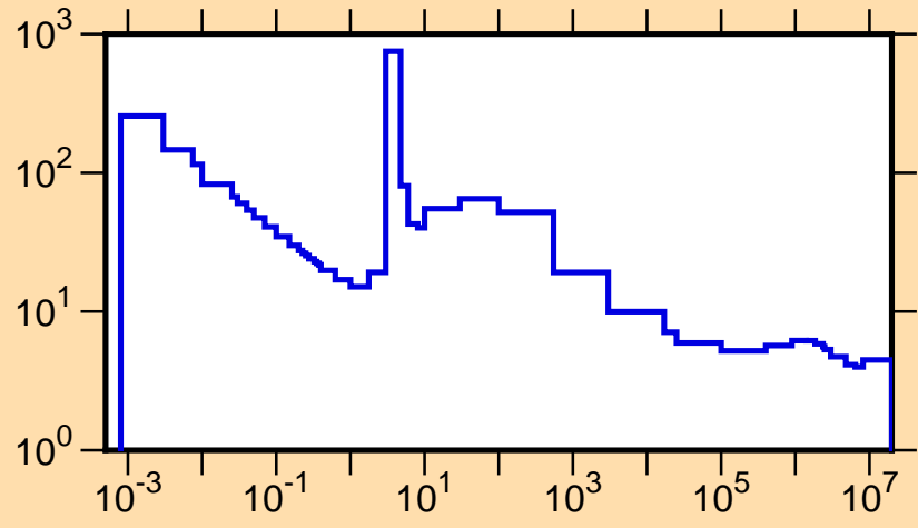
\sigma vs. E for ^{122}\text{Ba}(n,\text{tot.})
