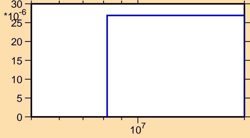
\sigma vs. E for ^{122}\text{Ba}(n,t)
