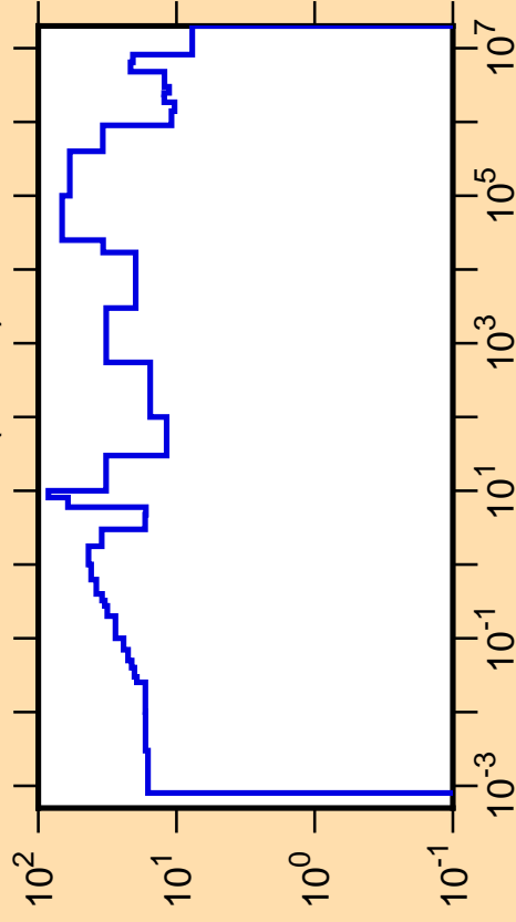
\Delta\sigma/\sigma vs. E for ^{122}\text{Ba}(n,\text{tot.})
