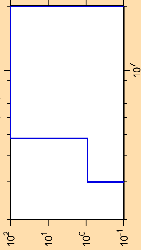
\Delta\sigma/\sigma vs. E for ^{122}\text{Ba}(n,d)
