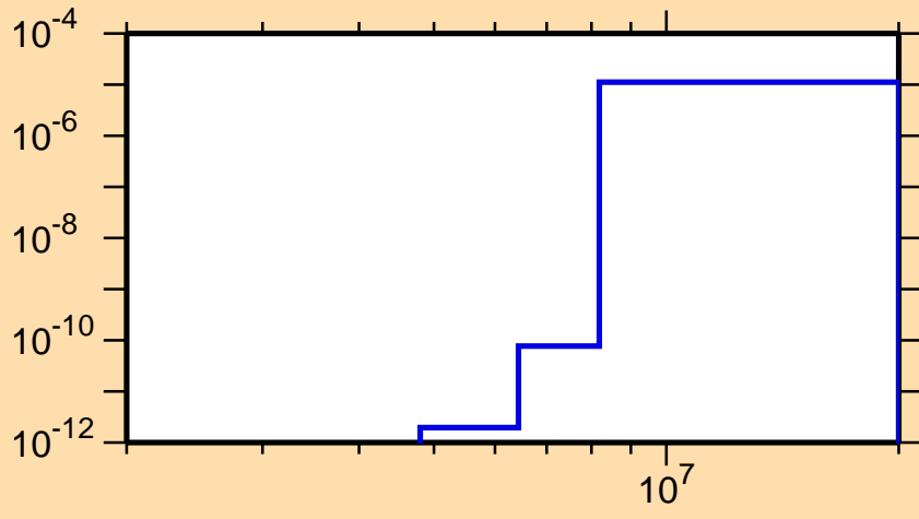
\sigma vs. E for ^{122}\text{Ba}(n,\text{He3})
