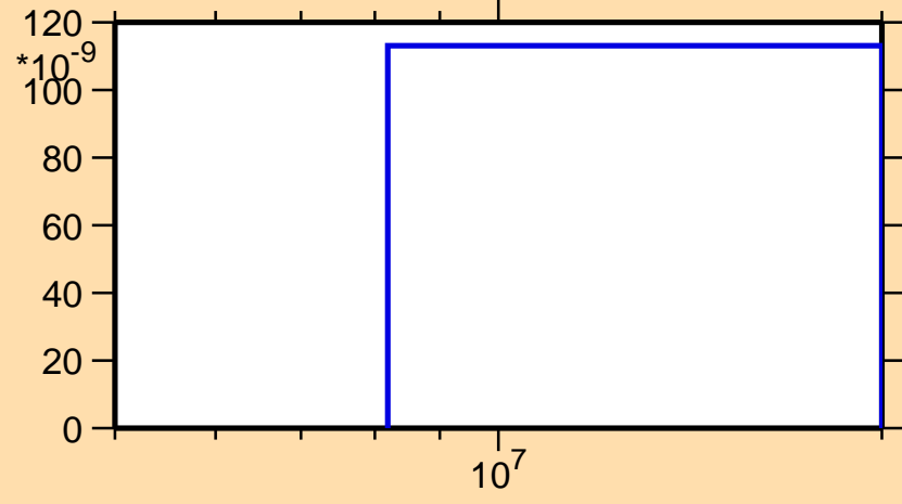
\sigma vs. E for ^{122}\text{Ba}(\text{mt } 45)
