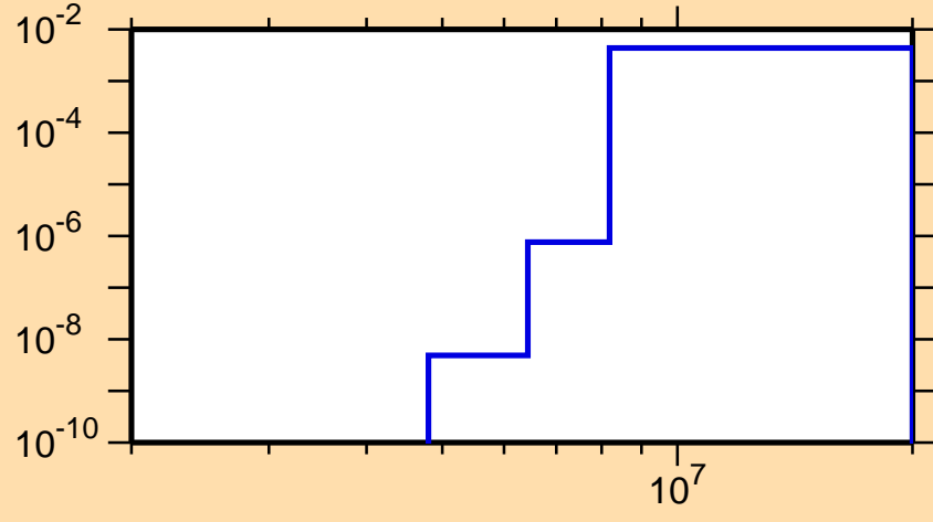
\sigma vs. E for ^{122}\text{Ba}(n,d)
