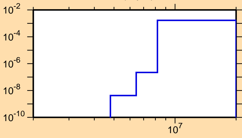
\sigma vs. E for ^{122}\text{Ba}(n,p\alpha)
