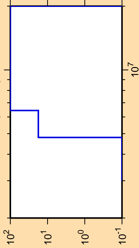
\Delta\sigma/\sigma vs. E for ^{122}\text{Ba}(n,\text{He3})
