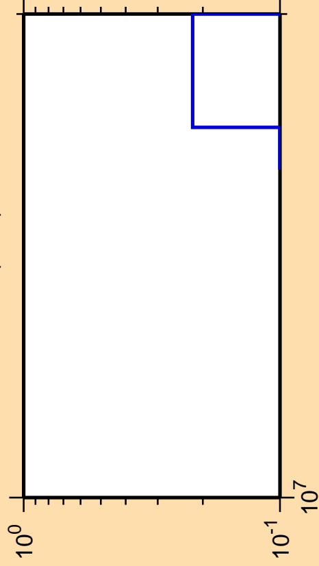
\Delta\sigma/\sigma vs. E for ^{123}\text{Ba}(n,nt)
