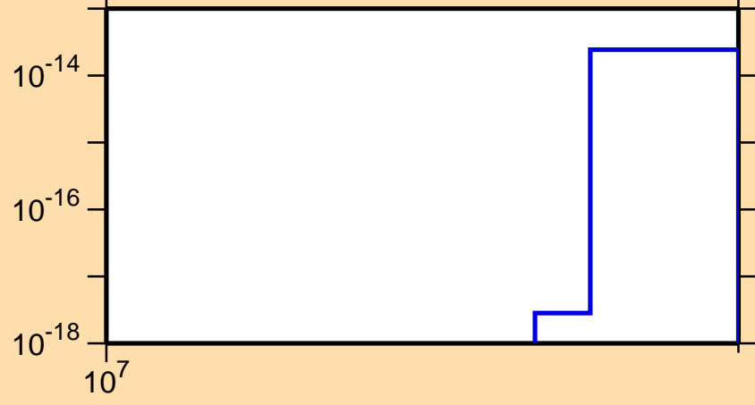
\sigma vs. E for ^{123}\text{Ba}(n,nt)
