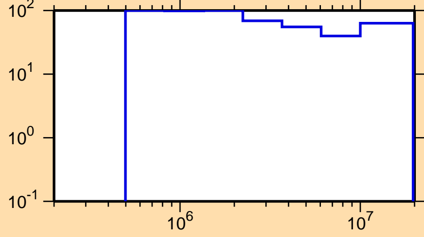
\Delta\sigma/\sigma vs. E for ^{123}\text{Ba}(n,n\text{cont.})
