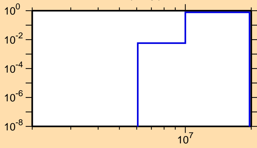
\sigma vs. E for ^{123}\text{Ba}(n,np)
