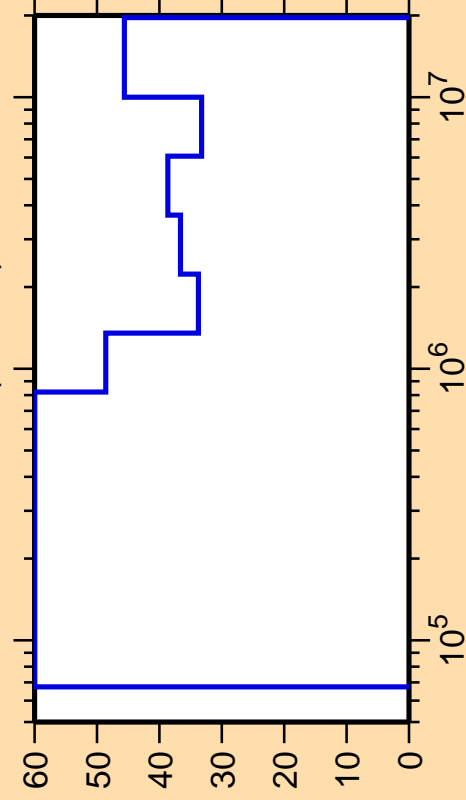
\Delta\sigma/\sigma vs. E for ^{123}\text{Ba}(n,\text{inel.})
