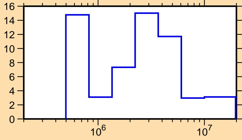
\Delta\sigma/\sigma vs. E for ^{123}\text{Ba}(n,el.)
