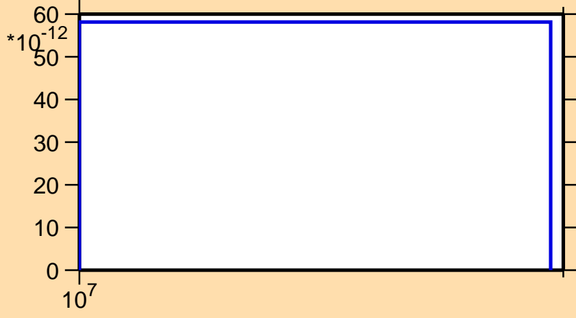
\sigma vs. E for ^{123}\text{Ba} (mt117)
