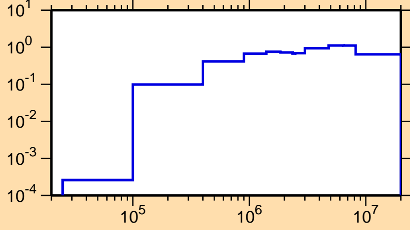
\sigma vs. E for ^{123}\text{Ba}(n,\text{inel.})
