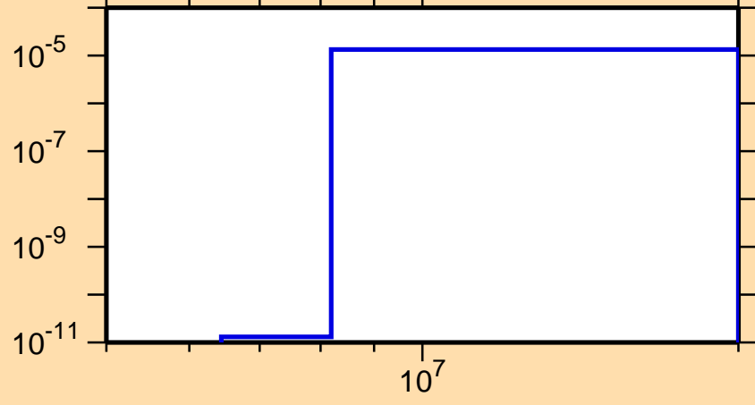
\sigma vs. E for ^{123}\text{Ba}(n,\text{He3})
