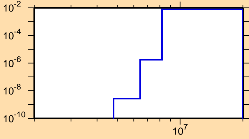
\sigma vs. E for ^{123}\text{Ba}(n,d)
