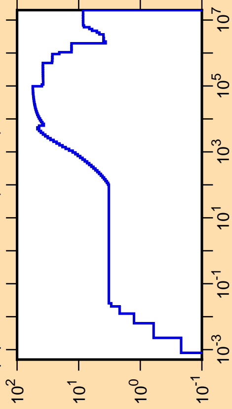
\Delta\mu/\mu vs. E for ^{124}\text{Ba}(\text{mt251})
