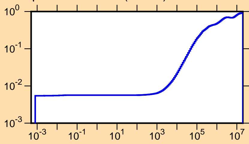
\mu vs. E for ^{124}\text{Ba}(\text{mt251})
