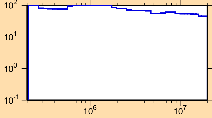
\Delta\sigma/\sigma vs. E for ^{124}\text{Ba}(n,n_1)
