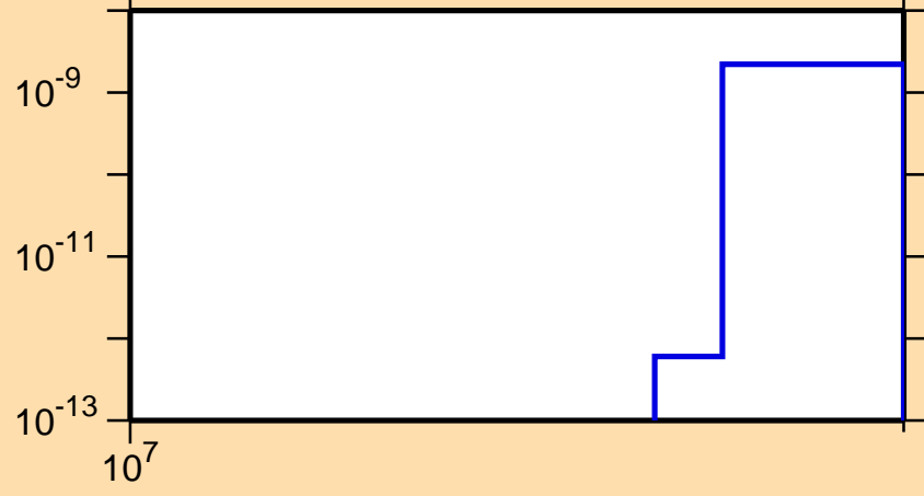
\sigma vs. E for ^{124}\text{Ba}(n,\text{pt})
