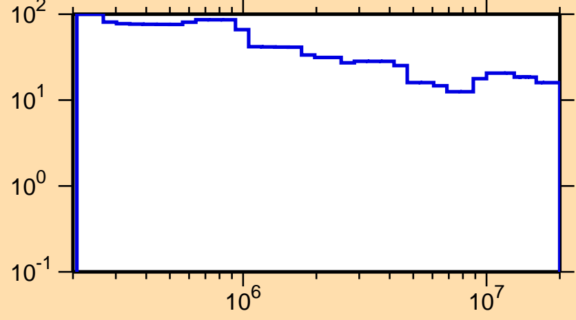
\Delta\sigma/\sigma vs. E for ^{124}\text{Ba}(n,\text{inel.})
