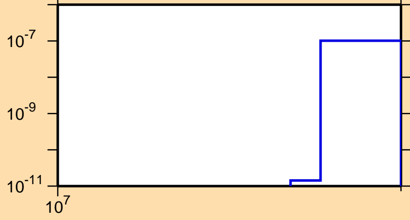
\sigma vs. E for ^{124}\text{Ba}(n,\text{nd})
