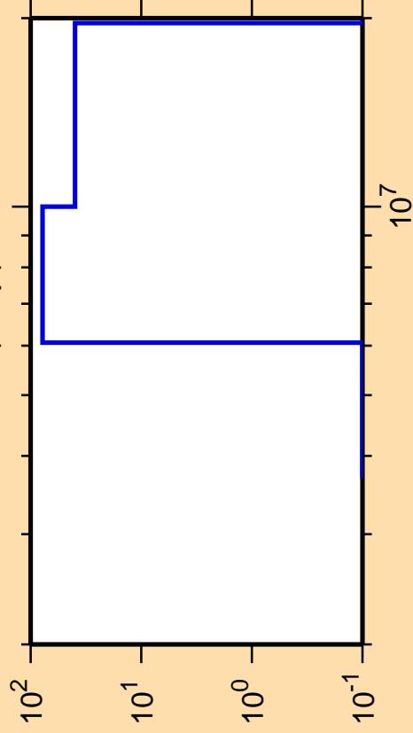
\Delta\sigma/\sigma vs. E for ^{124}\text{Ba}(n,np)
