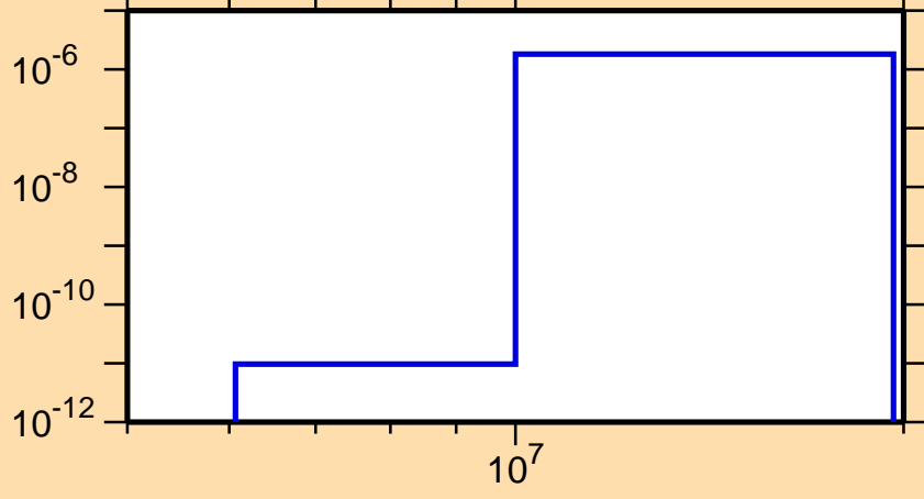
\sigma vs. E for ^{124}\text{Ba}(n,\text{He3})
