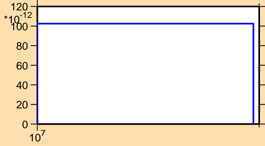
\sigma vs. E for ^{124}\text{Ba}(n,2n\alpha)
