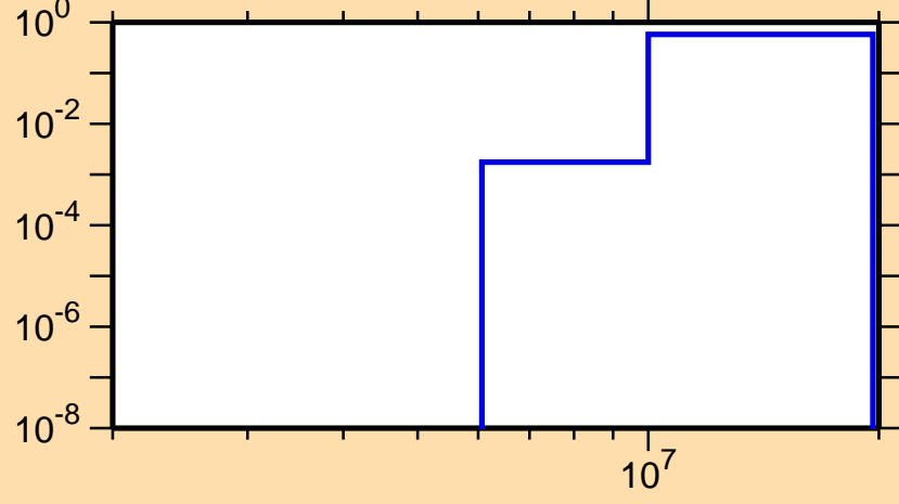
\sigma vs. E for ^{124}\text{Ba}(n,np)
