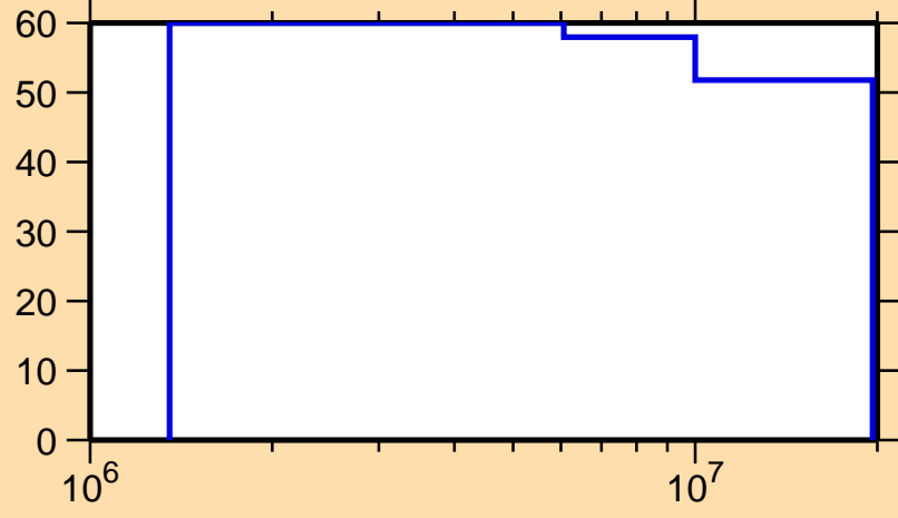
\Delta\sigma/\sigma vs. E for ^{124}\text{Ba}(n,n_1)
