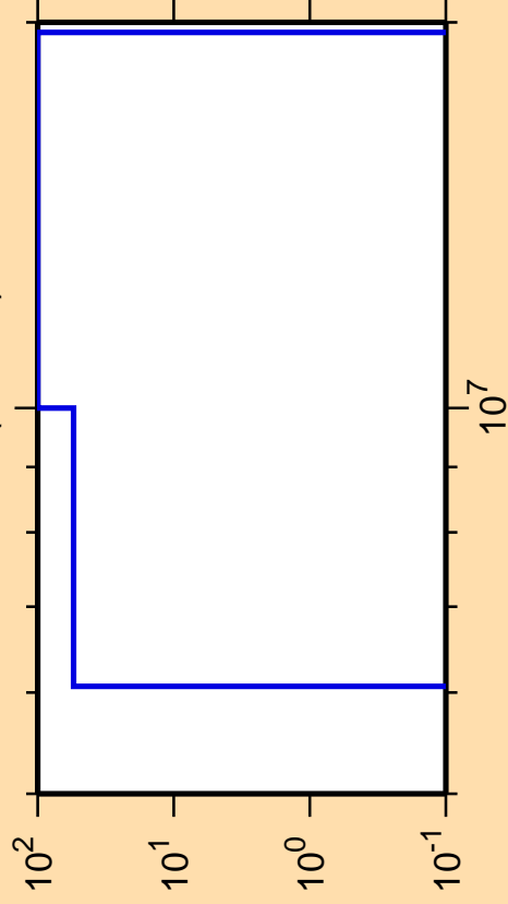
\Delta\sigma/\sigma vs. E for ^{124}\text{Ba}(n,\text{He3})
