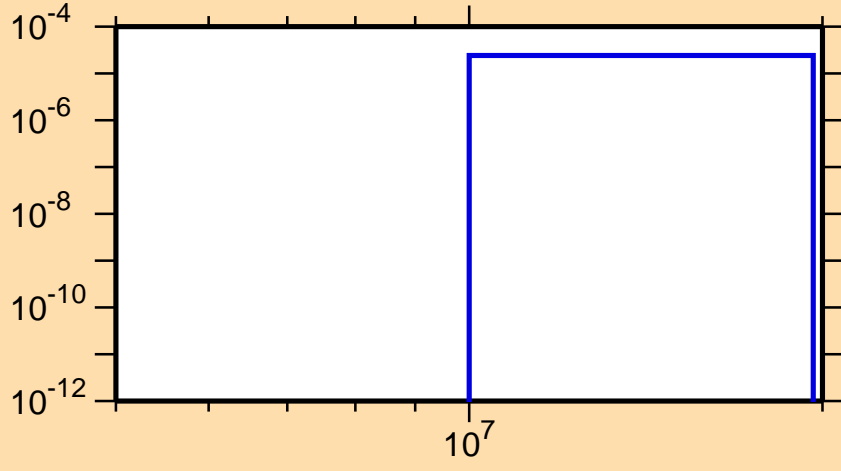
\sigma vs. E for ^{124}\text{Ba}(n,t)
