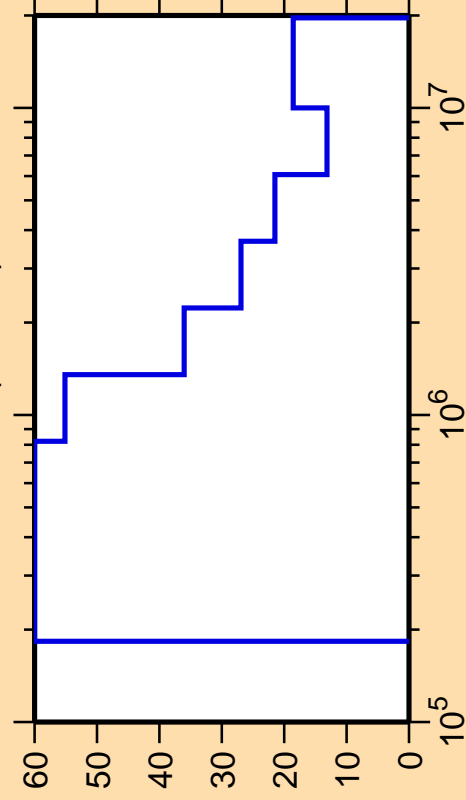
\Delta\sigma/\sigma vs. E for ^{124}\text{Ba}(n,\text{inel.})
