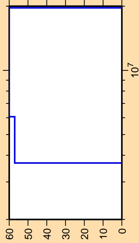
\Delta\sigma/\sigma vs. E for ^{124}\text{Ba}(n,d)
