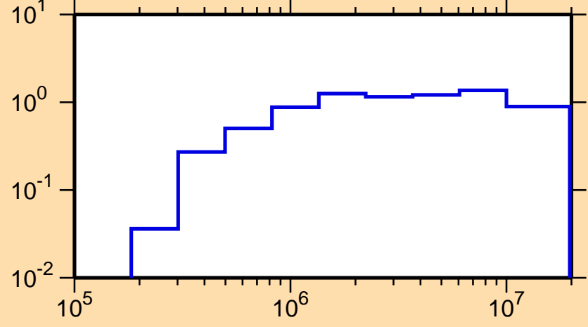
\sigma vs. E for ^{124}\text{Ba}(n,\text{inel.})
