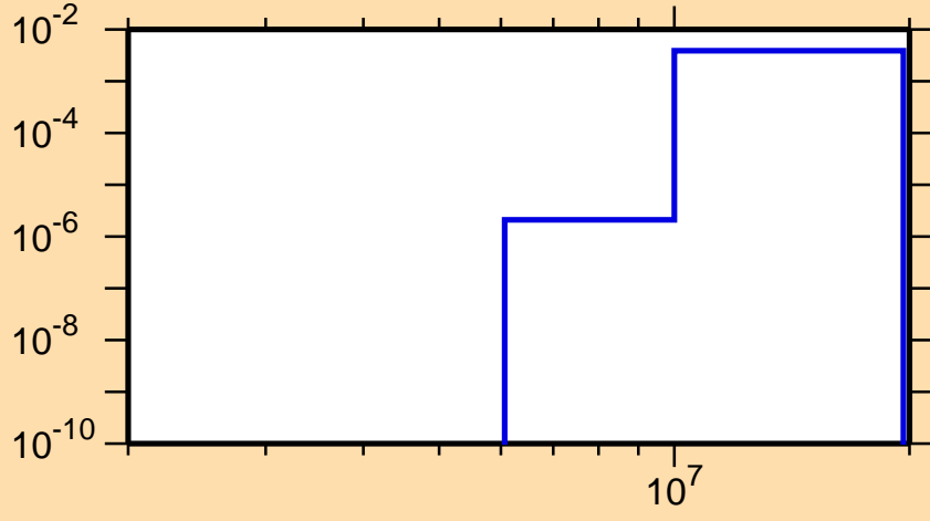
\sigma vs. E for ^{124}\text{Ba}(n,d)
