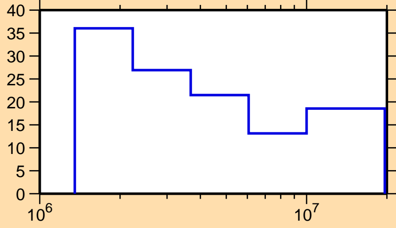
\Delta\sigma/\sigma vs. E for ^{124}\text{Ba}(n,\text{inel.})
