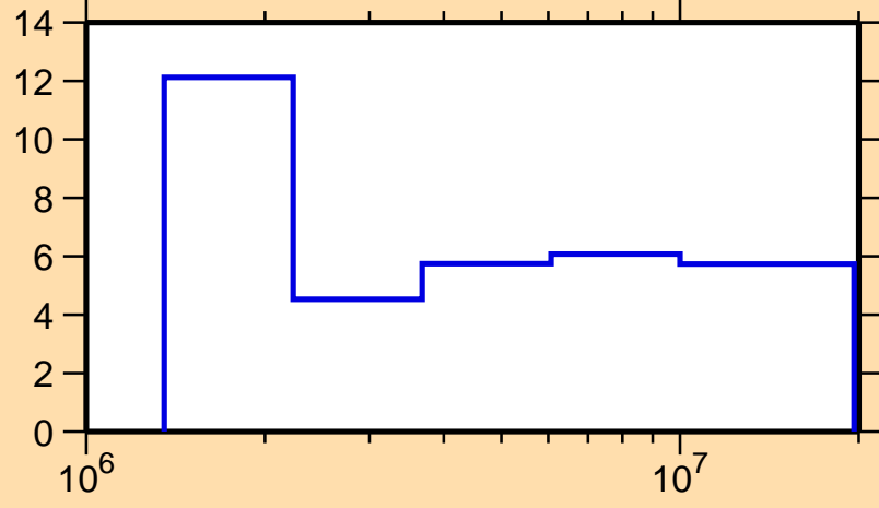
\Delta\sigma/\sigma vs. E for ^{124}\text{Ba}(n,n\text{onel.})
