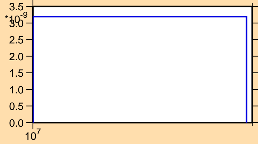
\sigma vs. E for ^{124}\text{Ba}(n,2np)
