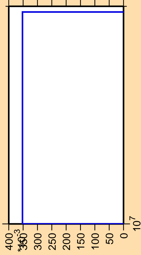
\Delta\sigma/\sigma vs. E for ^{124}\text{Ba} (mt 34)
