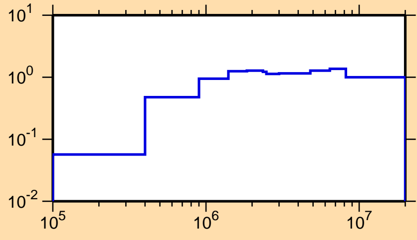
\sigma vs. E for ^{124}\text{Ba}(n,\text{inel.})
