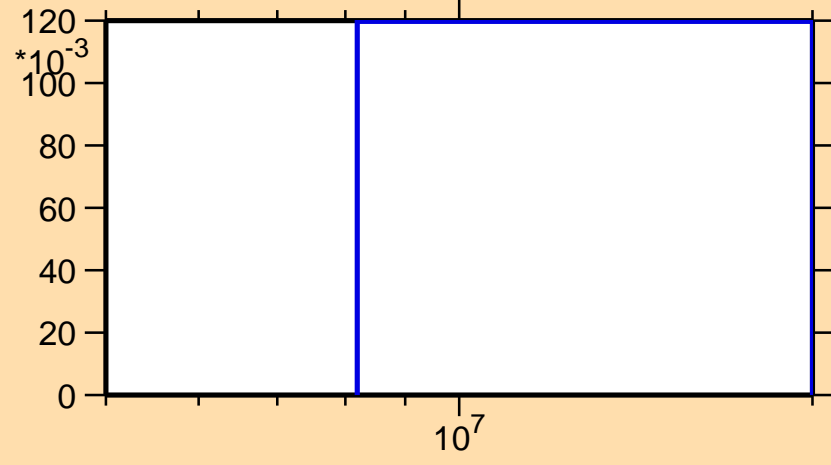
\sigma vs. E for ^{124}\text{Ba}(n,2n)
