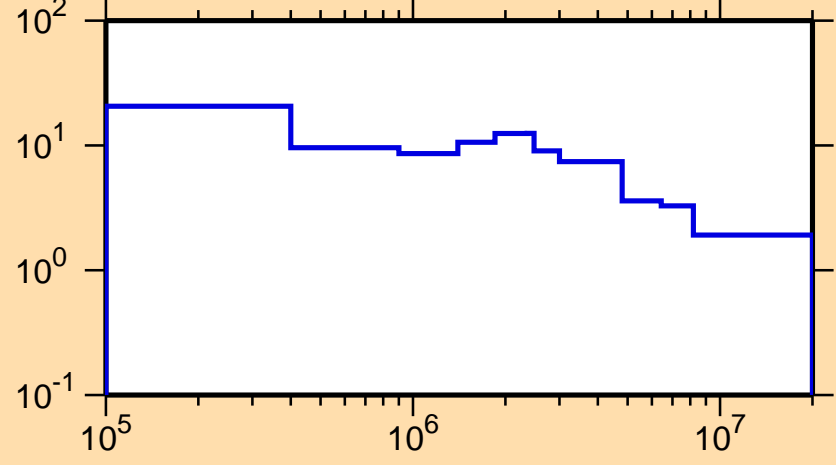
\Delta\sigma/\sigma vs. E for ^{124}\text{Ba}(n,\text{tot.})
